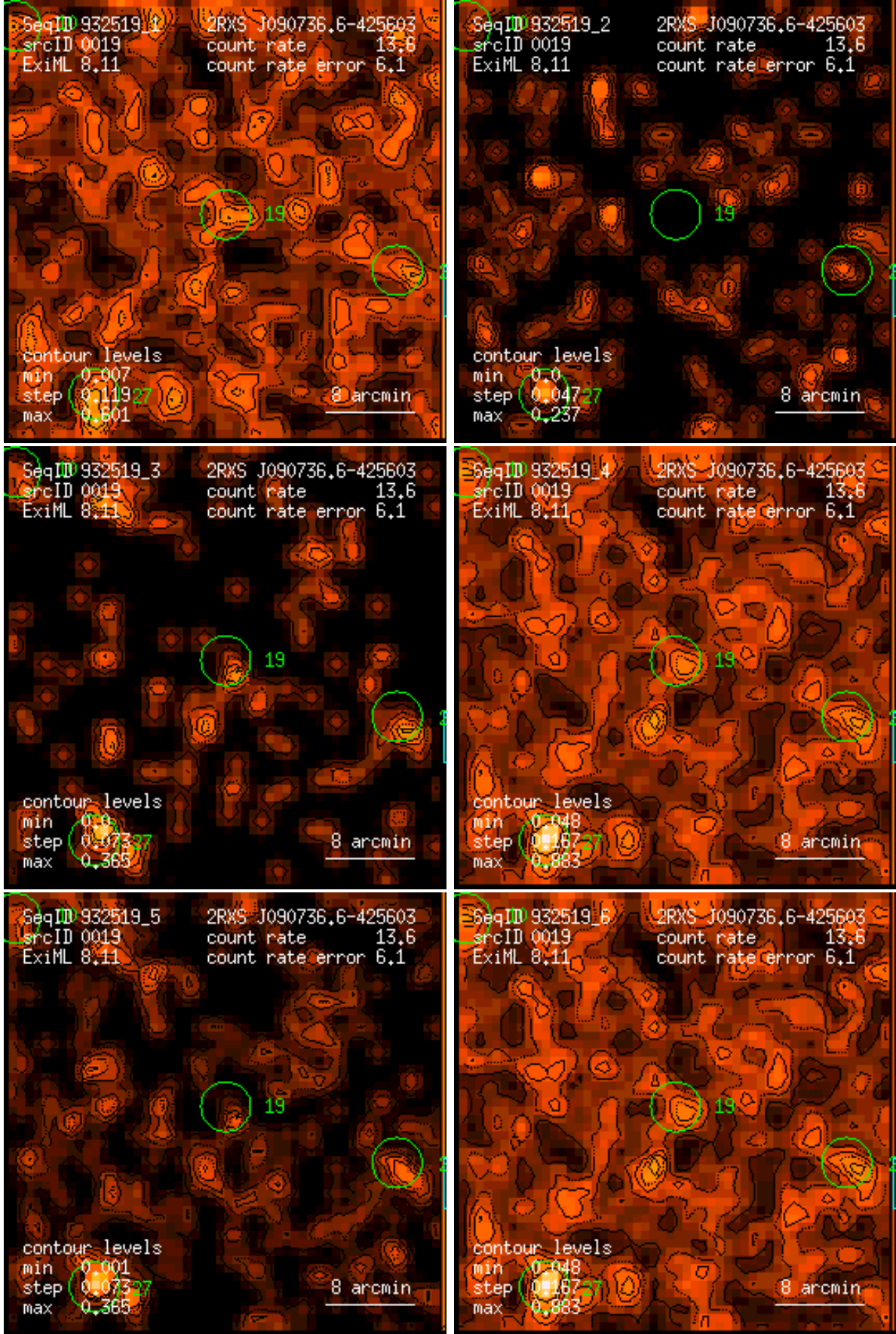
Figure 19: RASS 932519: detection 0019: band rate images, Gaussian filter: (1) PSPC channels 11 – 41, (2) 52 – 90, (3) 91 – 201, (4) 11 – 235, (5) 52 – 201, (6) 11 – 201. Broad band rates in counts/ks. Band rate contour levels in counts/ks/arcmin 2 .
