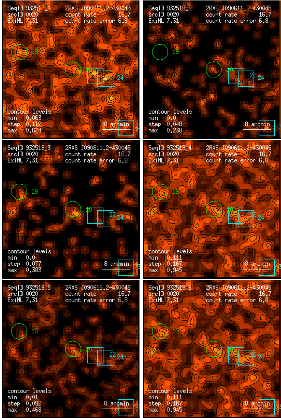
Figure 20: RASS 932519: detection 0020: band rate images, Gaussian filter: (1) PSPC channels 11 – 41, (2) 52 – 90, (3) 91 – 201, (4) 11 – 235, (5) 52 – 201, (6) 11 – 201. Broad band rates in counts/ks. Band rate contour levels in counts/ks/arcmin 2 .
