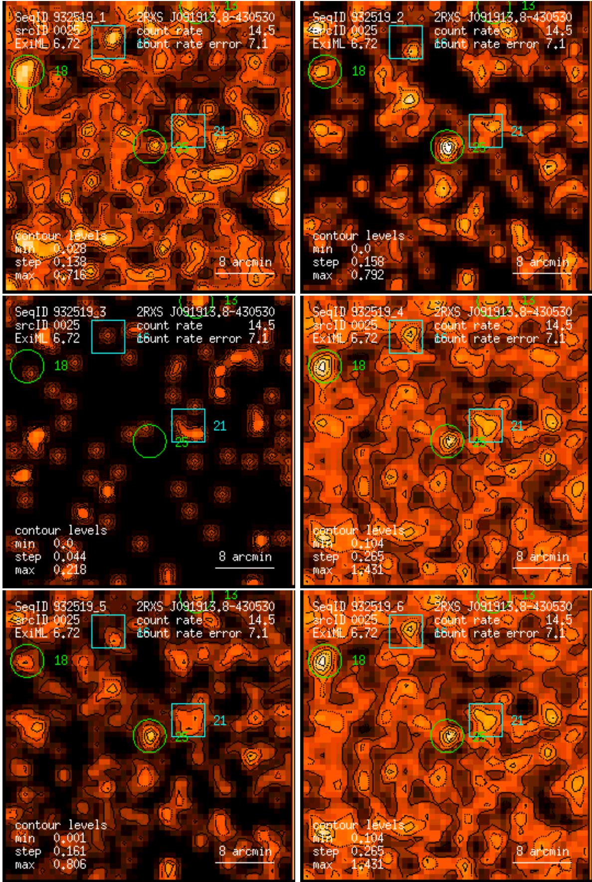
Figure 25: RASS 932519: detection 0025: band rate images, Gaussian filter: (1) PSPC channels 11 – 41, (2) 52 – 90, (3) 91 – 201, (4) 11 – 235, (5) 52 – 201, (6) 11 – 201. Broad band rates in counts/ks. Band rate contour levels in counts/ks/arcmin 2 .
