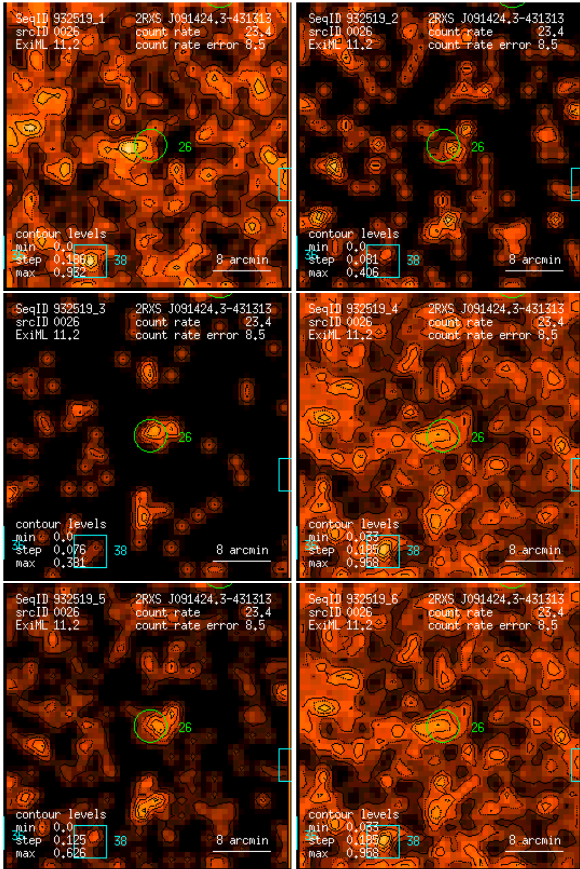
Figure 26: RASS 932519: detection 0026: band rate images, Gaussian filter: (1) PSPC channels 11 – 41, (2) 52 – 90, (3) 91 – 201, (4) 11 – 235, (5) 52 – 201, (6) 11 – 201. Broad band rates in counts/ks. Band rate contour levels in counts/ks/arcmin 2 .
