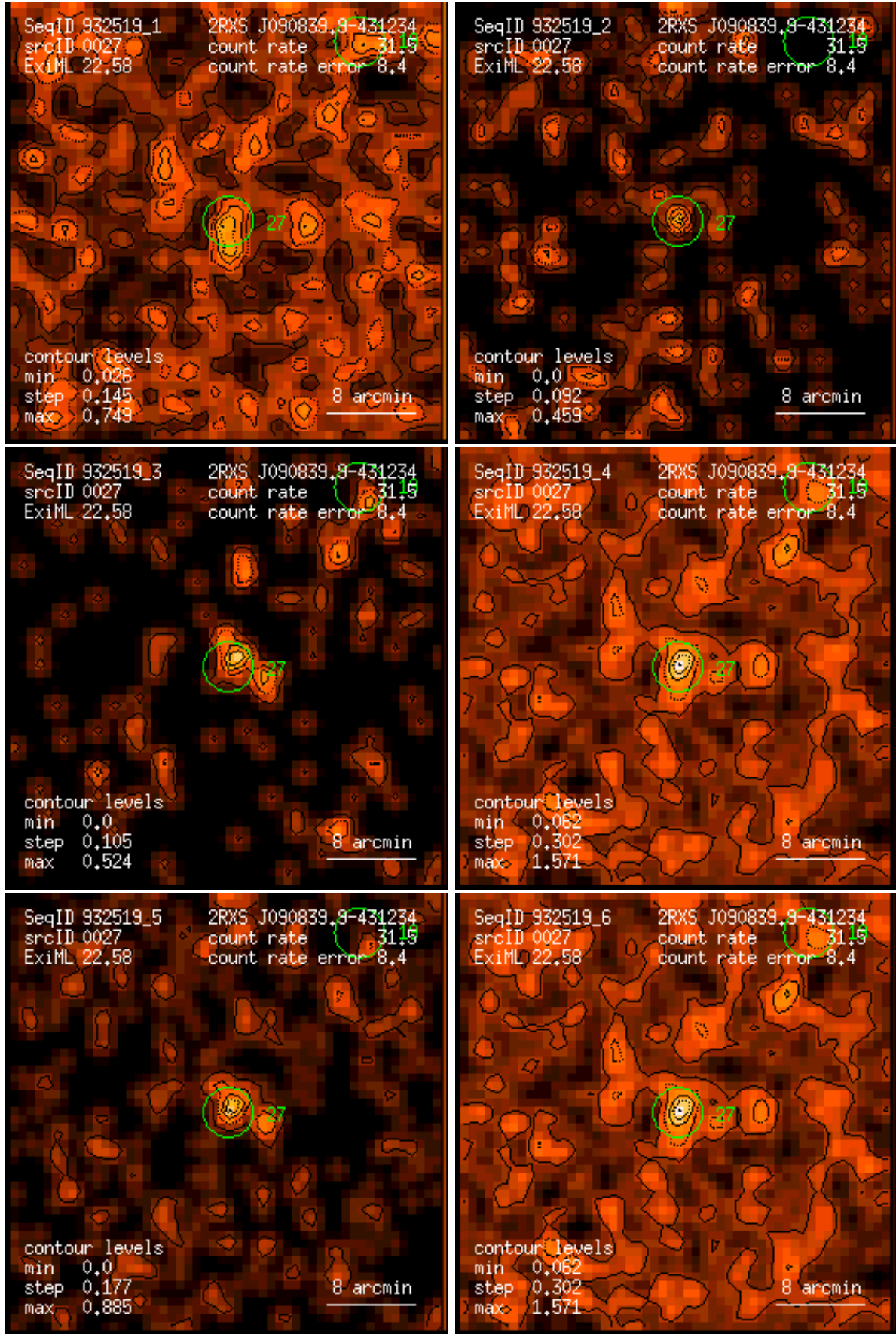
Figure 27: RASS 932519: detection 0027: band rate images, Gaussian filter: (1) PSPC channels 11 – 41, (2) 52 – 90, (3) 91 – 201, (4) 11 – 235, (5) 52 – 201, (6) 11 – 201. Broad band rates in counts/ks. Band rate contour levels in counts/ks/arcmin 2 .
