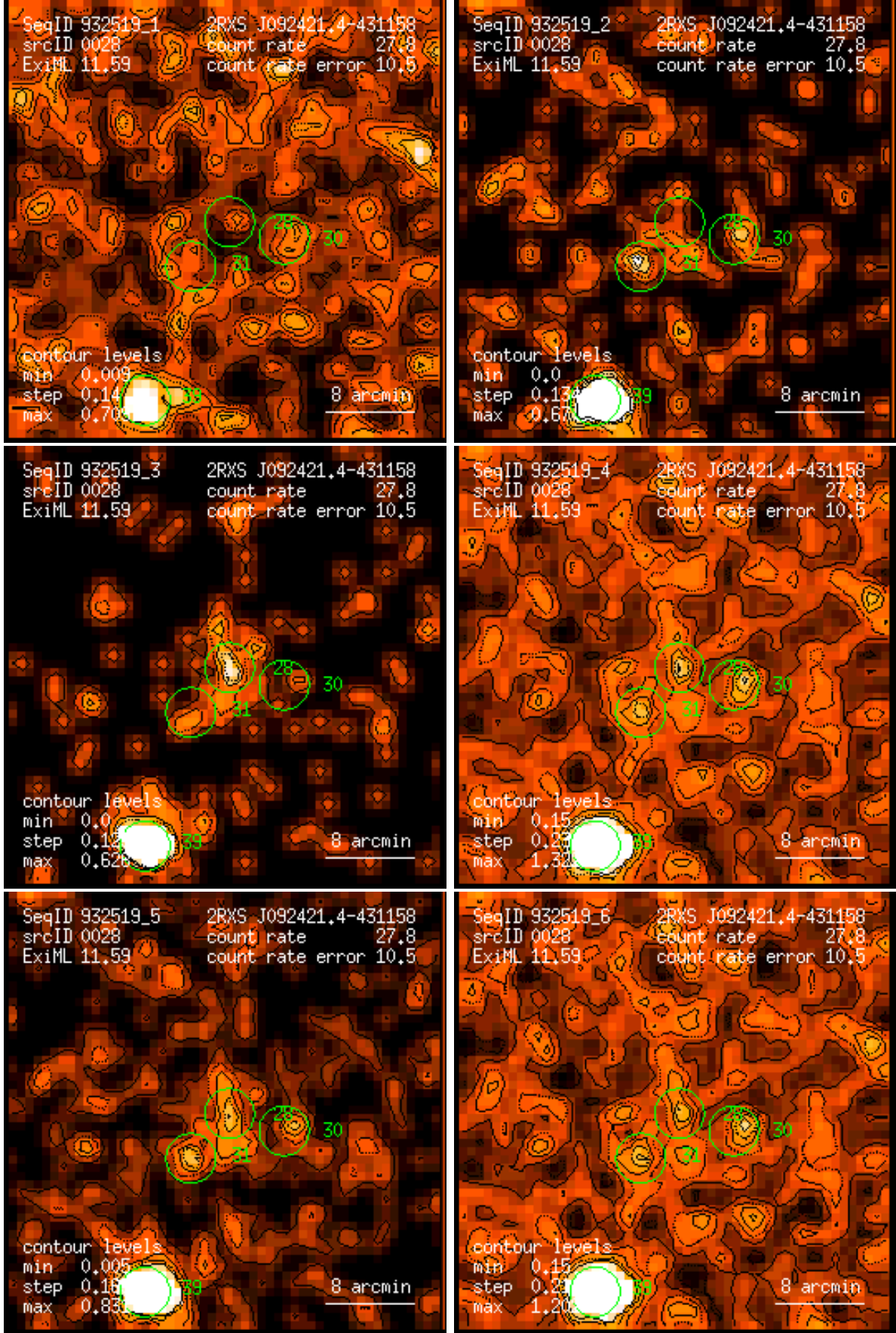
Figure 28: RASS 932519: detection 0028: band rate images, Gaussian filter: (1) PSPC channels 11 – 41, (2) 52 – 90, (3) 91 – 201, (4) 11 – 235, (5) 52 – 201, (6) 11 – 201. Broad band rates in counts/ks. Band rate contour levels in counts/ks/arcmin 2 .
