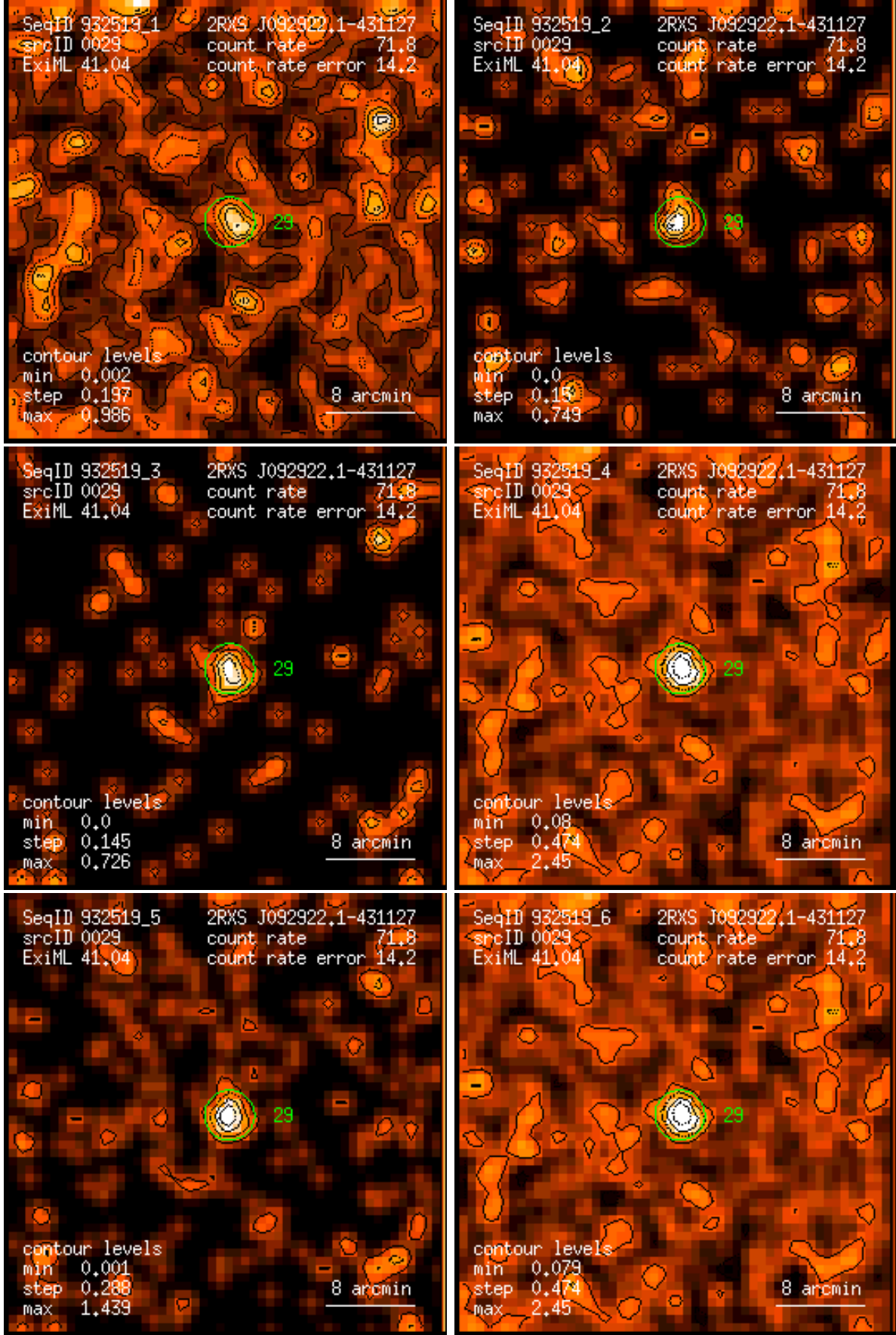
Figure 29: RASS 932519: detection 0029: band rate images, Gaussian filter: (1) PSPC channels 11 – 41, (2) 52 – 90, (3) 91 – 201, (4) 11 – 235, (5) 52 – 201, (6) 11 – 201. Broad band rates in counts/ks. Band rate contour levels in counts/ks/arcmin 2 .
