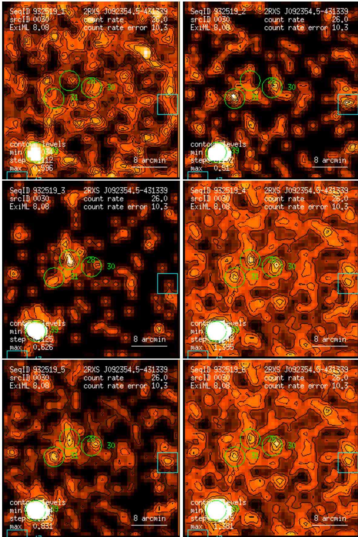
Figure 30: RASS 932519: detection 0030: band rate images, Gaussian filter: (1) PSPC channels 11 – 41, (2) 52 – 90, (3) 91 – 201, (4) 11 – 235, (5) 52 – 201, (6) 11 – 201. Broad band rates in counts/ks. Band rate contour levels in counts/ks/arcmin 2 .
