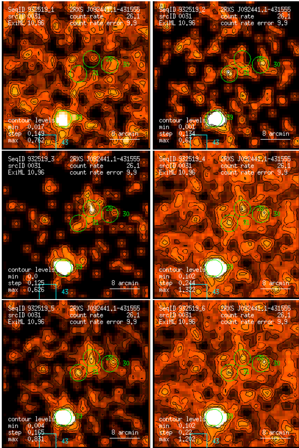
Figure 31: RASS 932519: detection 0031: band rate images, Gaussian filter: (1) PSPC channels 11 – 41, (2) 52 – 90, (3) 91 – 201, (4) 11 – 235, (5) 52 – 201, (6) 11 – 201. Broad band rates in counts/ks. Band rate contour levels in counts/ks/arcmin 2 .
