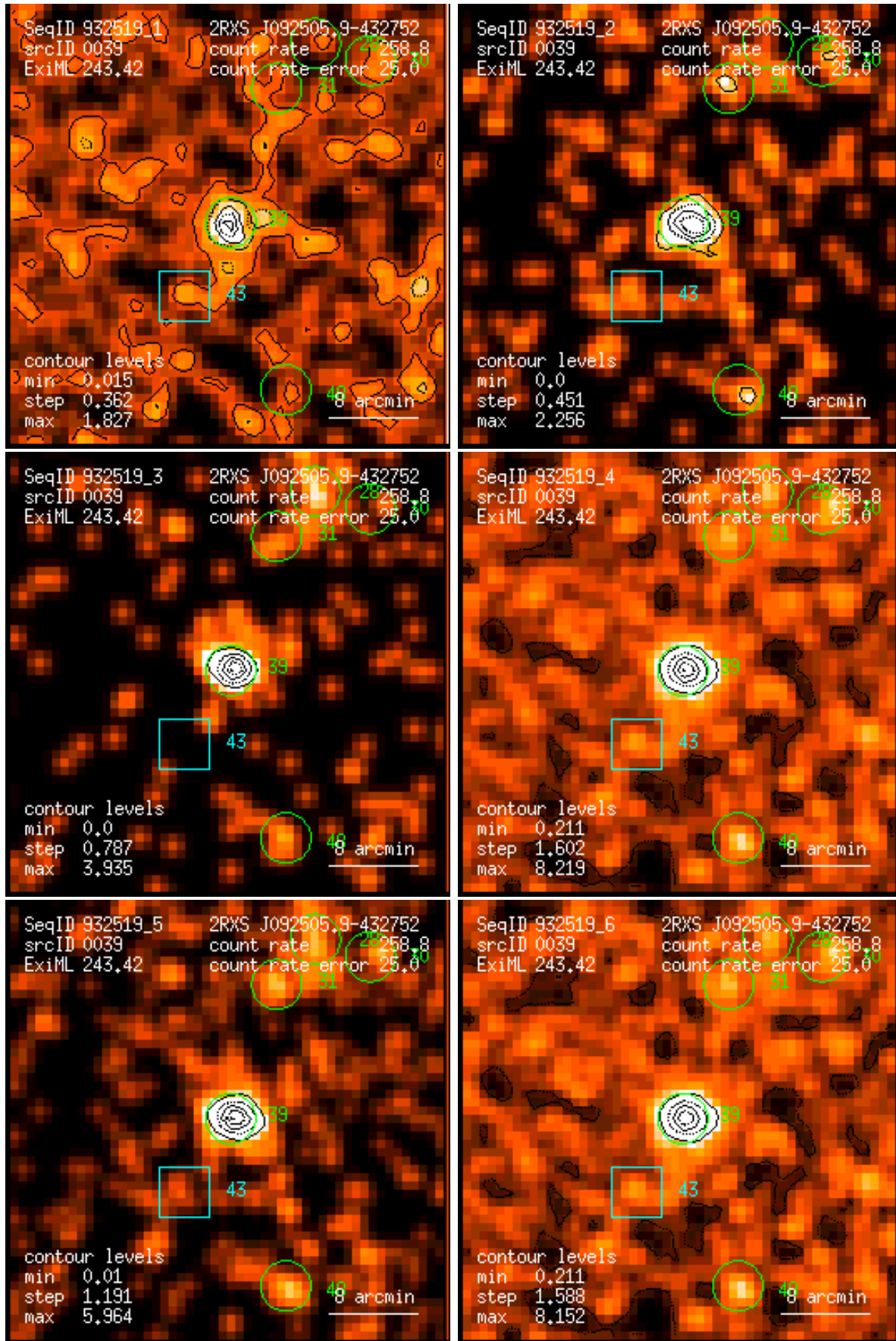
Figure 39: RASS 932519: detection 0039: band rate images, Gaussian filter: (1) PSPC channels 11 – 41, (2) 52 – 90, (3) 91 – 201, (4) 11 – 235, (5) 52 – 201, (6) 11 – 201. Broad band rates in counts/ks. Band rate contour levels in counts/ks/arcmin 2 .
