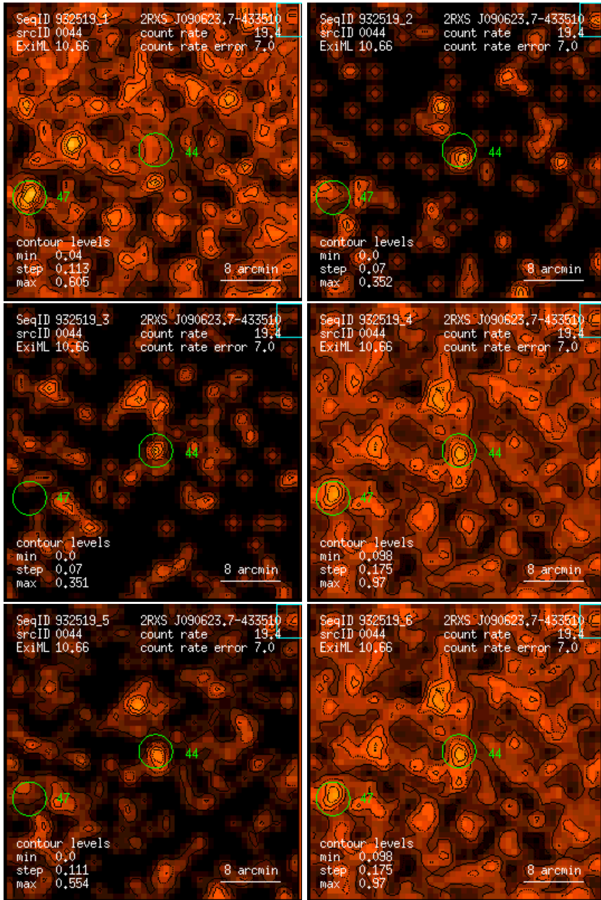
Figure 44: RASS 932519: detection 0044: band rate images, Gaussian filter: (1) PSPC channels 11 – 41, (2) 52 – 90, (3) 91 – 201, (4) 11 – 235, (5) 52 – 201, (6) 11 – 201. Broad band rates in counts/ks. Band rate contour levels in counts/ks/arcmin 2 .
