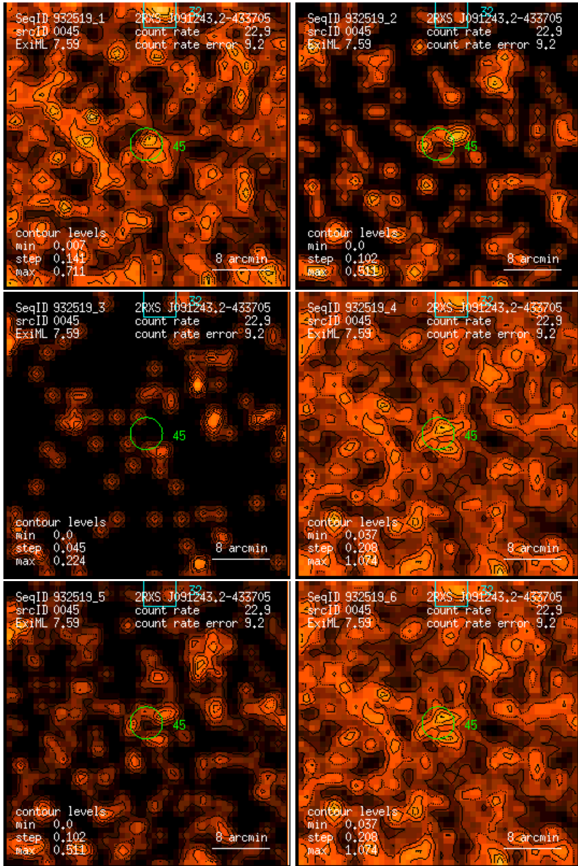
Figure 45: RASS 932519: detection 0045: band rate images, Gaussian filter: (1) PSPC channels 11 – 41, (2) 52 – 90, (3) 91 – 201, (4) 11 – 235, (5) 52 – 201, (6) 11 – 201. Broad band rates in counts/ks. Band rate contour levels in counts/ks/arcmin 2 .
