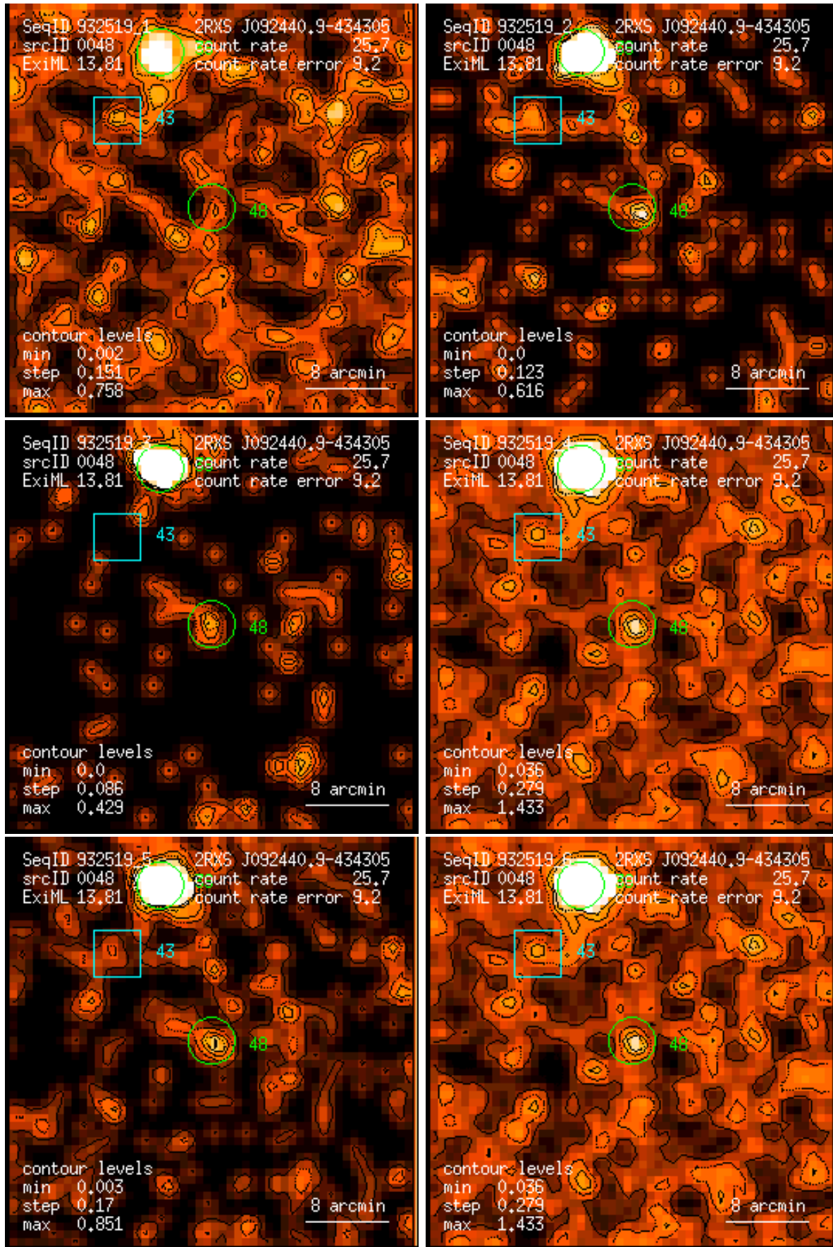
Figure 48: RASS 932519: detection 0048: band rate images, Gaussian filter: (1) PSPC channels 11 – 41, (2) 52 – 90, (3) 91 – 201, (4) 11 – 235, (5) 52 – 201, (6) 11 – 201. Broad band rates in counts/ks. Band rate contour levels in counts/ks/arcmin 2 .
