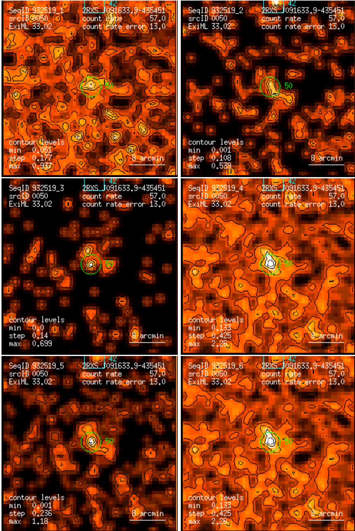
Figure 50: RASS 932519: detection 0050: band rate images, Gaussian filter: (1) PSC channels 11 – 41, (2) 52 – 90, (3) 91 – 201, (4) 11 – 235, (5) 52 – 201, (6) 11 – 201. Broad band rates in counts/ks. Band rate contour levels in counts/ks/arcmin 2 .
