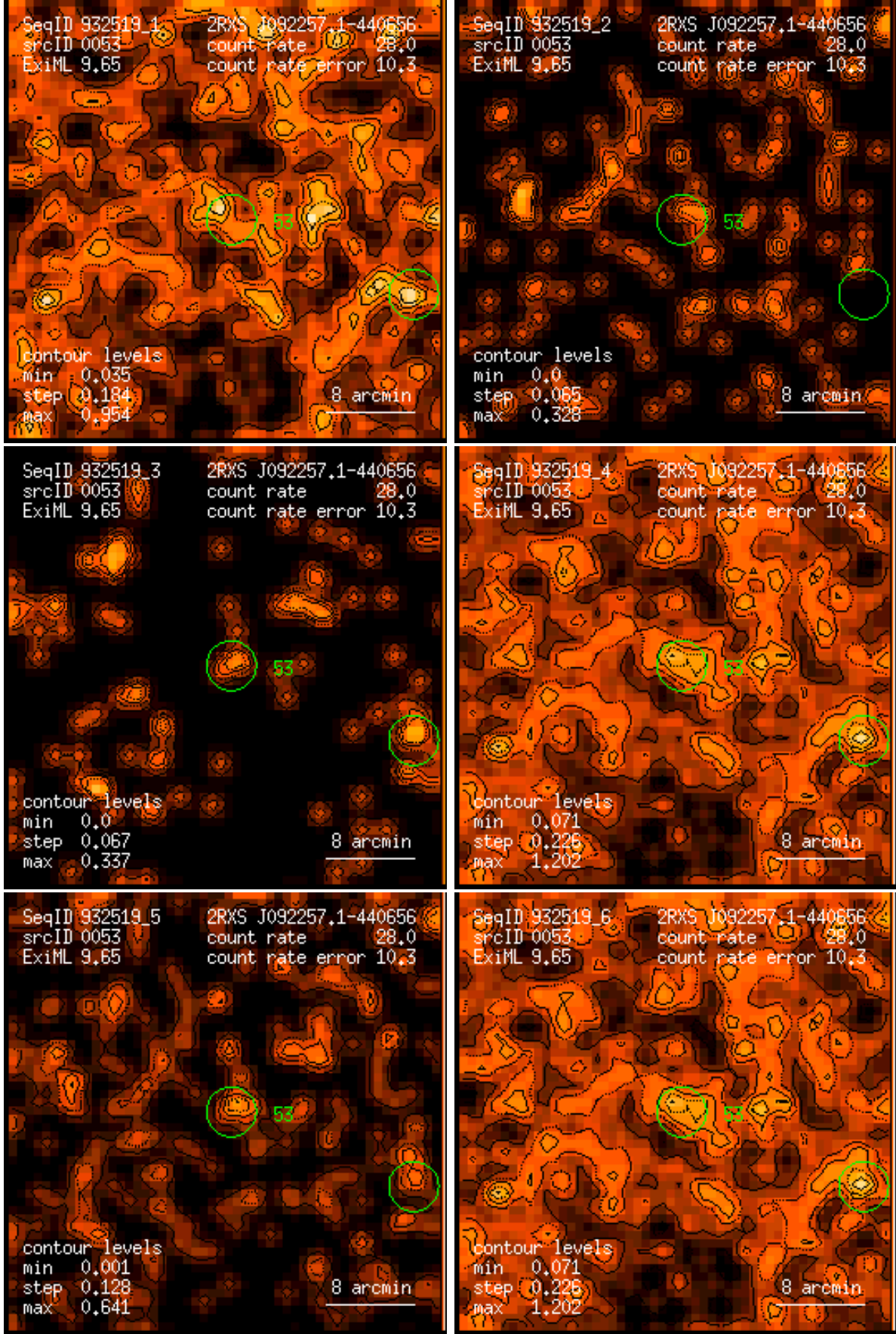
Figure 53: RASS 932519: detection 0053: band rate images, Gaussian filter: (1) PSPC channels 11 – 41, (2) 52 – 90, (3) 91 – 201, (4) 11 – 235, (5) 52 – 201, (6) 11 – 201. Broad band rates in counts/ks. Band rate contour levels in counts/ks/arcmin 2 .
