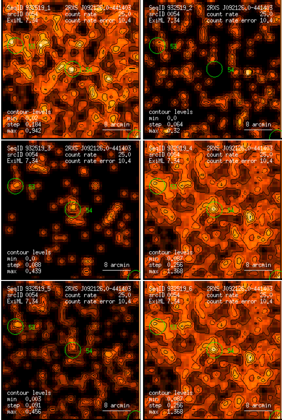
Figure 54: RASS 932519: detection 0054: band rate images, Gaussian filter: (1) PSPC channels 11 – 41, (2) 52 – 90, (3) 91 – 201, (4) 11 – 235, (5) 52 – 201, (6) 11 – 201. Broad band rates in counts/ks. Band rate contour levels in counts/ks/arcmin 2 .
