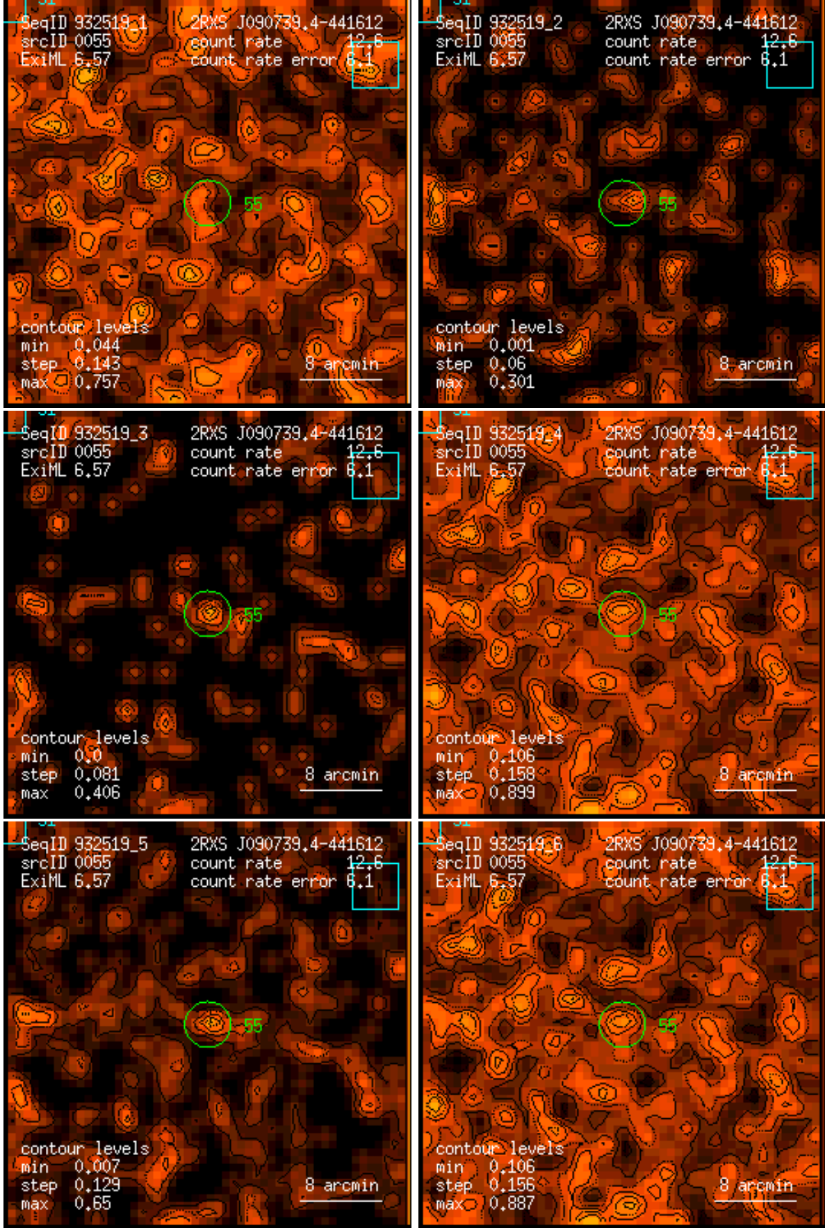
Figure 55: RASS 932519: detection 0055: band rate images, Gaussian filter: (1) PSPC channels 11 – 41, (2) 52 – 90, (3) 91 – 201, (4) 11 – 235, (5) 52 – 201, (6) 11 – 201. Broad band rates in counts/ks. Band rate contour levels in counts/ks/arcmin 2 .
