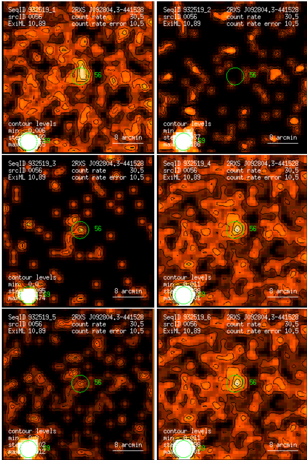
Figure 56: RASS 932519: detection 0056: band rate images, Gaussian filter: (1) PSPC channels 11 – 41, (2) 52 – 90, (3) 91 – 201, (4) 11 – 235, (5) 52 – 201, (6) 11 – 201. Broad band rates in counts/ks. Band rate contour levels in counts/ks/arcmin 2 .
