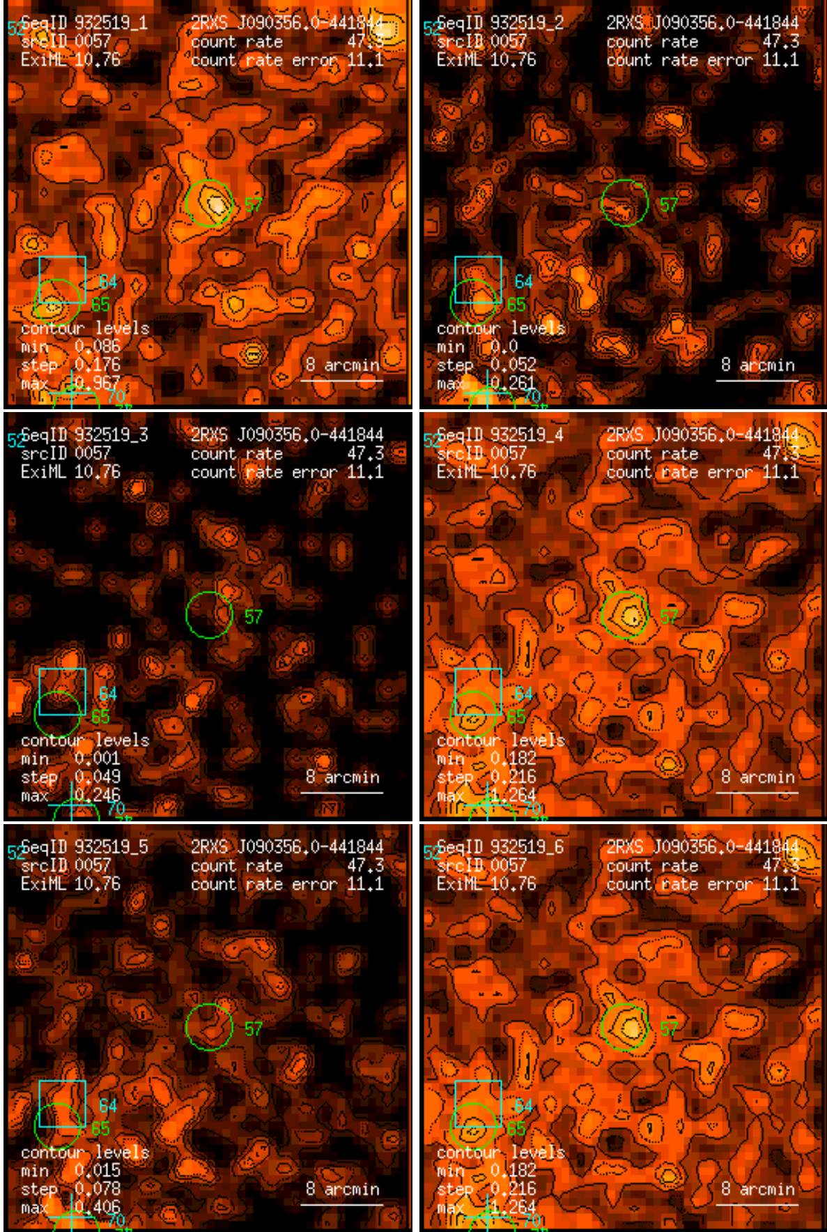
Figure 57: RASS 932519: detection 0057: band rate images, Gaussian filter: (1) PSPC channels 11 – 41, (2) 52 – 90, (3) 91 – 201, (4) 11 – 235, (5) 52 – 201, (6) 11 – 201. Broad band rates in counts/ks. Band rate contour levels in counts/ks/arcmin 2 .
