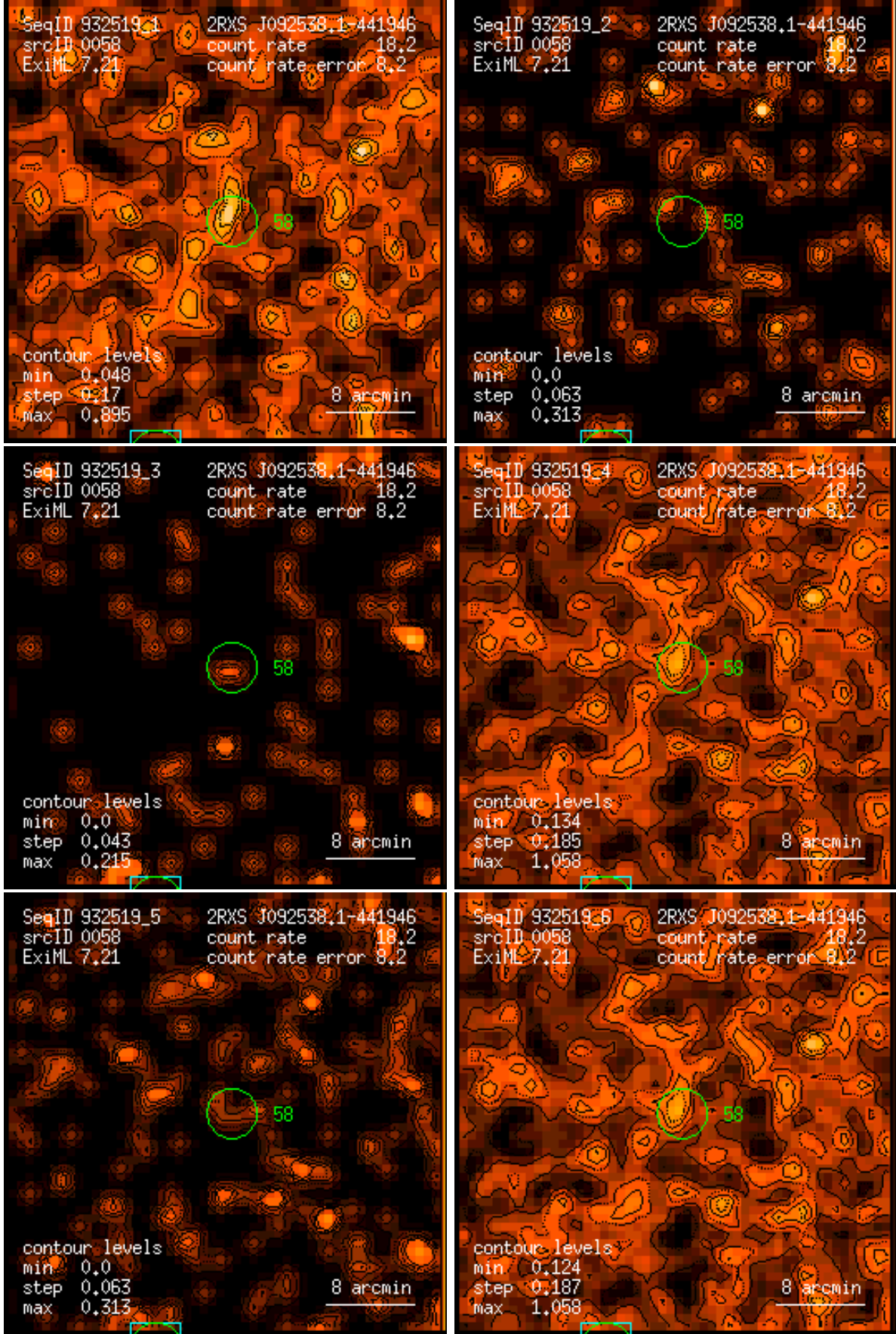
Figure 58: RASS 932519: detection 0058: band rate images, Gaussian filter: (1) PSPC channels 11 – 41, (2) 52 – 90, (3) 91 – 201, (4) 11 – 235, (5) 52 – 201, (6) 11 – 201. Broad band rates in counts/ks. Band rate contour levels in counts/ks/arcmin 2 .
