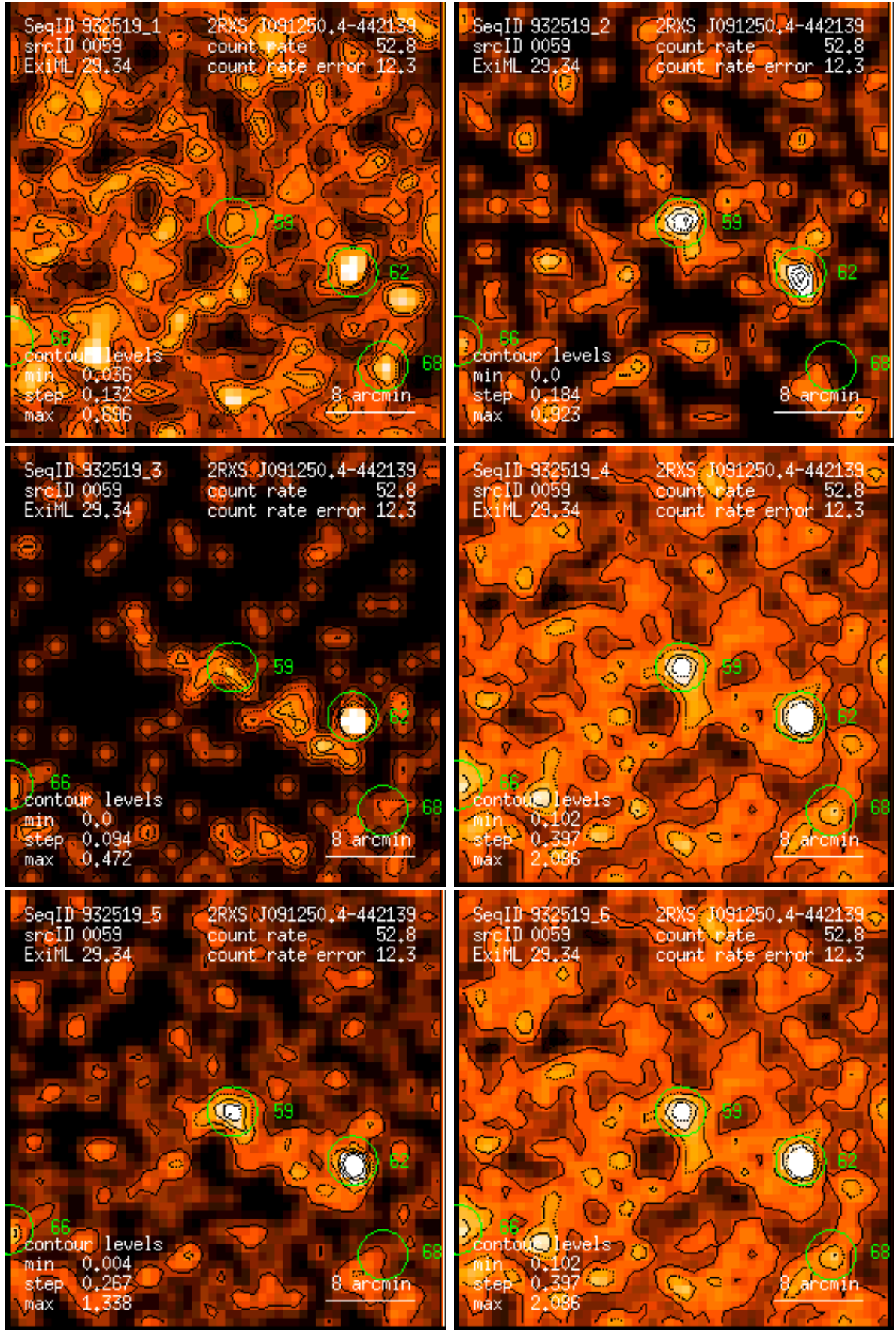
Figure 59: RASS 932519: detection 0059: band rate images, Gaussian filter: (1) PSPC channels 11 – 41, (2) 52 – 90, (3) 91 – 201, (4) 11 – 235, (5) 52 – 201, (6) 11 – 201. Broad band rates in counts/ks. Band rate contour levels in counts/ks/arcmin 2 .
