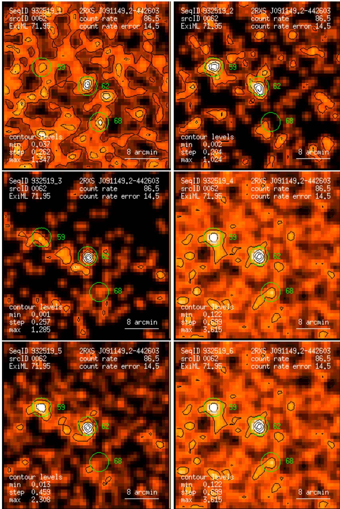
Figure 62: RASS 932519: detection 0062: band rate images, Gaussian filter: (1) PSPC channels 11 – 41, (2) 52 – 90, (3) 91 – 201, (4) 11 – 235, (5) 52 – 201, (6) 11 – 201. Broad band rates in counts/ks. Band rate contour levels in counts/ks/arcmin 2 .
