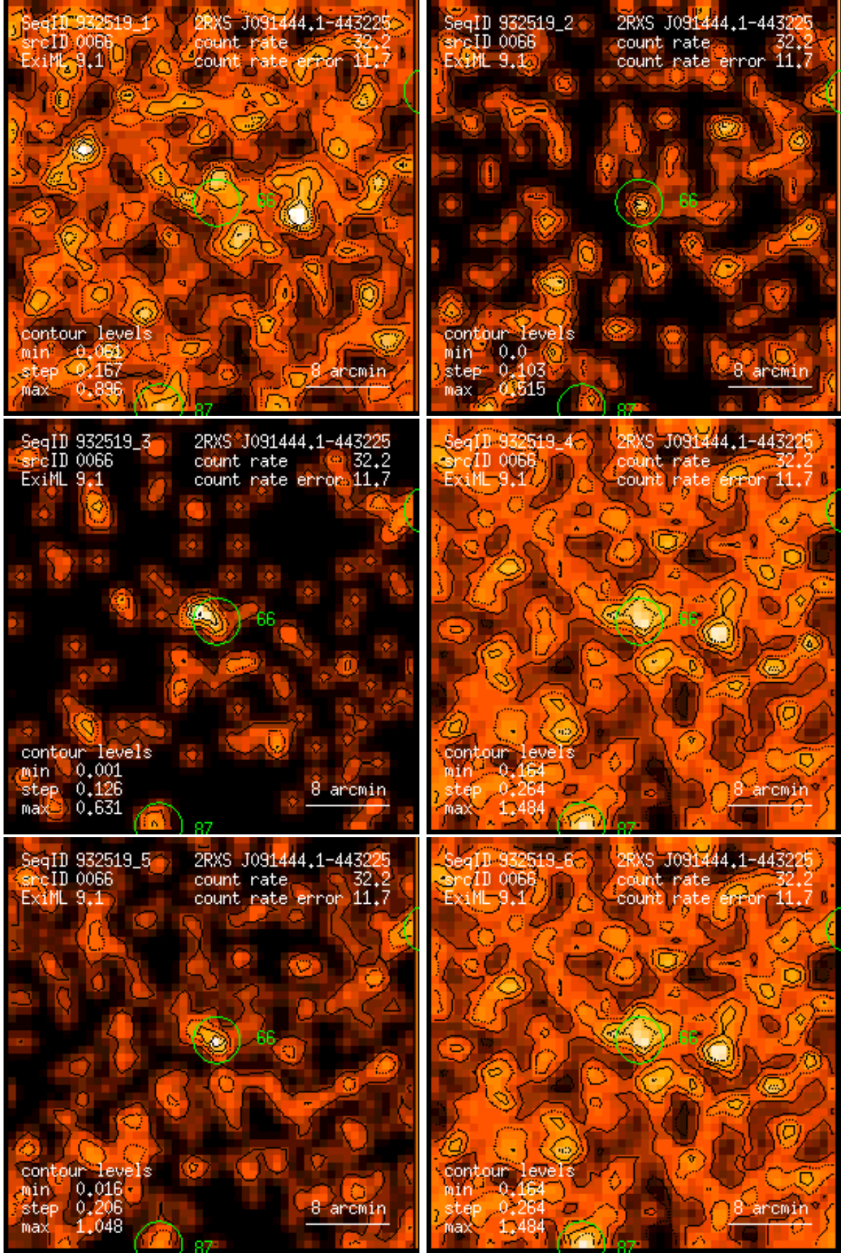
Figure 66: RASS 932519: detection 0066: band rate images, Gaussian filter: (1) PSPC channels 11 – 41, (2) 52 – 90, (3) 91 – 201, (4) 11 – 235, (5) 52 – 201, (6) 11 – 201. Broad band rates in counts/ks. Band rate contour levels in counts/ks/arcmin 2 .
