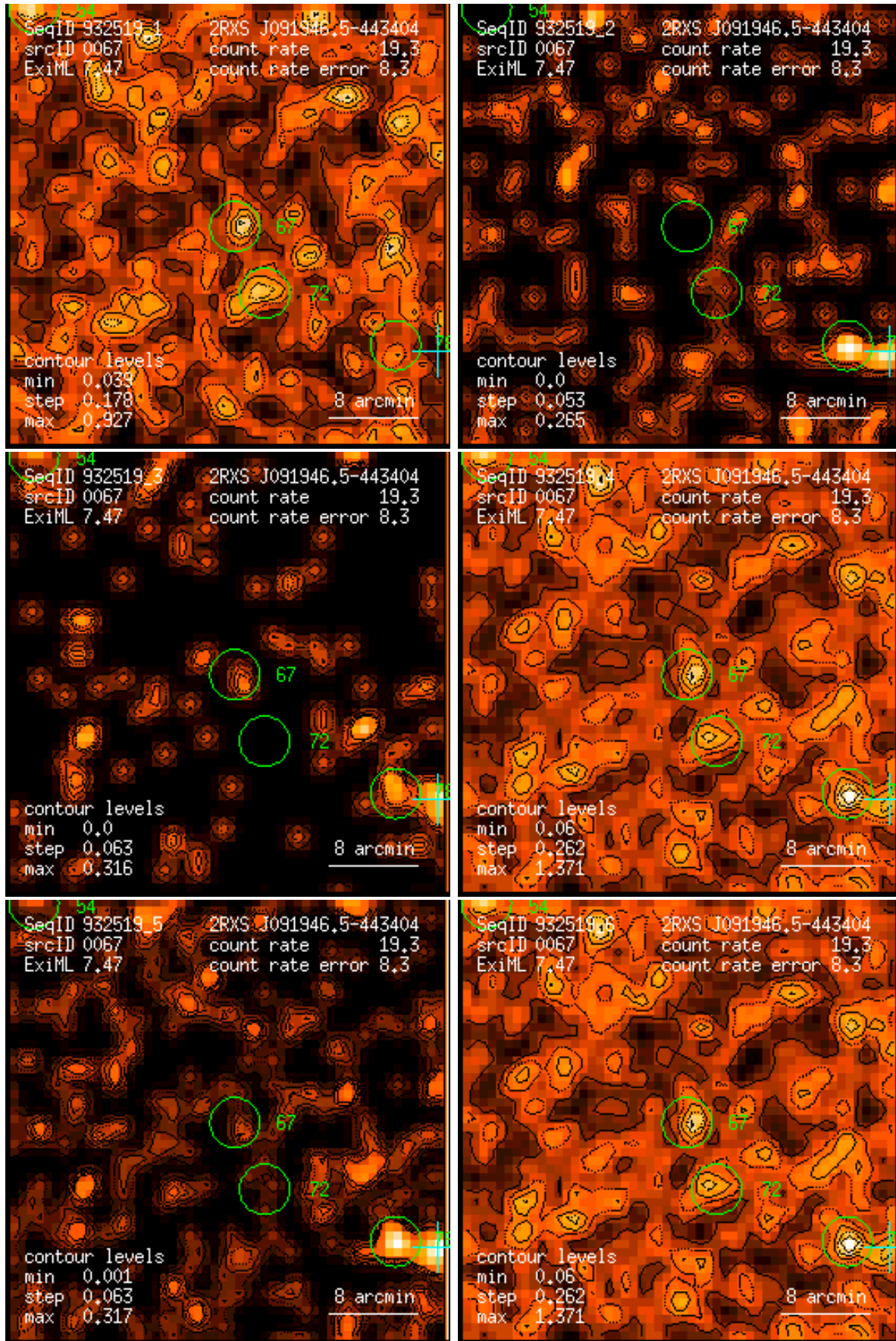
Figure 67: RASS 932519: detection 0067: band rate images, Gaussian filter: (1) PSPC channels 11 – 41, (2) 52 – 90, (3) 91 – 201, (4) 11 – 235, (5) 52 – 201, (6) 11 – 201. Broad band rates in counts/ks. Band rate contour levels in counts/ks/arcmin 2 .
