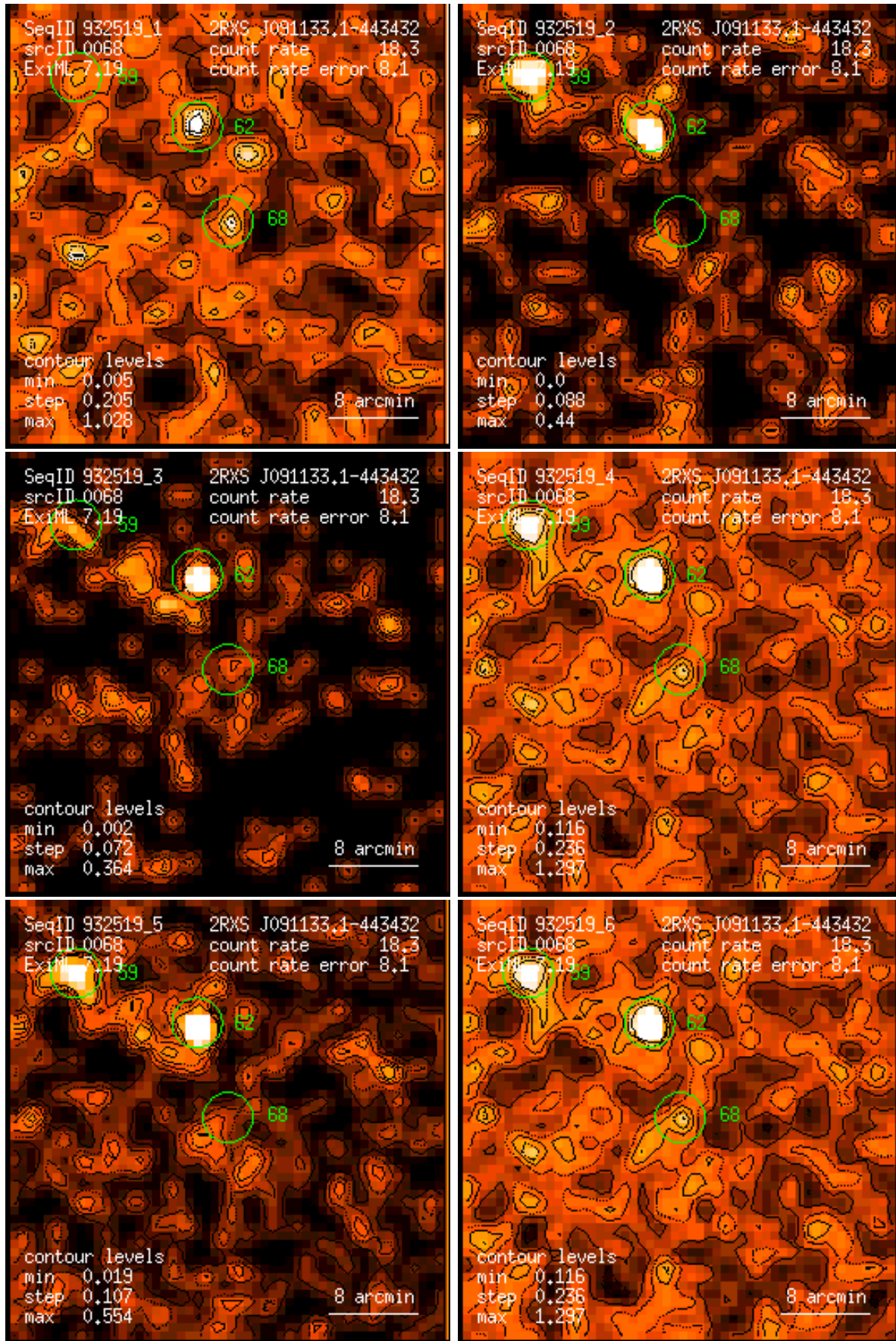
Figure 68: RASS 932519: detection 0068: band rate images, Gaussian filter: (1) PSPC channels 11 – 41, (2) 52 – 90, (3) 91 – 201, (4) 11 – 235, (5) 52 – 201, (6) 11 – 201. Broad band rates in counts/ks. Band rate contour levels in counts/ks/arcmin 2 .
