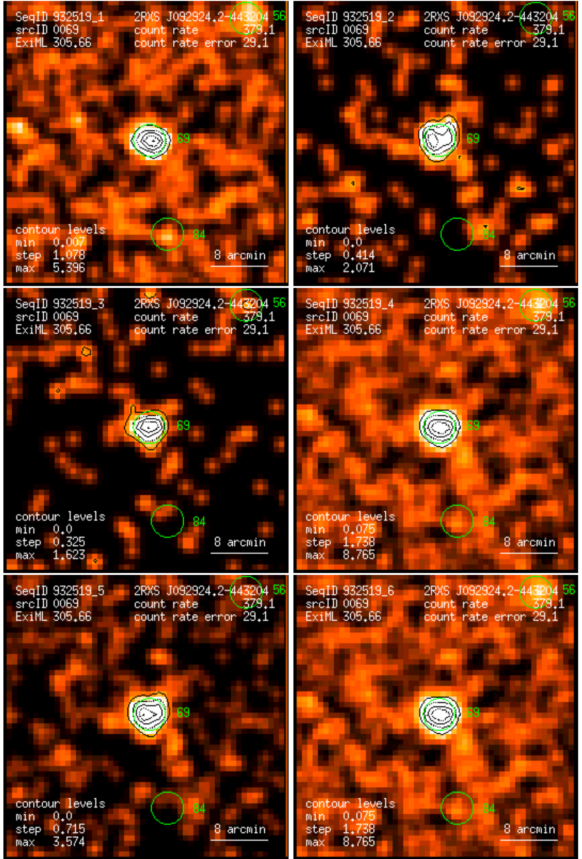
Figure 69: RASS 932519: detection 0069: band rate images, Gaussian filter: (1) PSPC channels 11 – 41, (2) 52 – 90, (3) 91 – 201, (4) 11 – 235, (5) 52 – 201, (6) 11 – 201. Broad band rates in counts/ks. Band rate contour levels in counts/ks/arcmin 2 .
