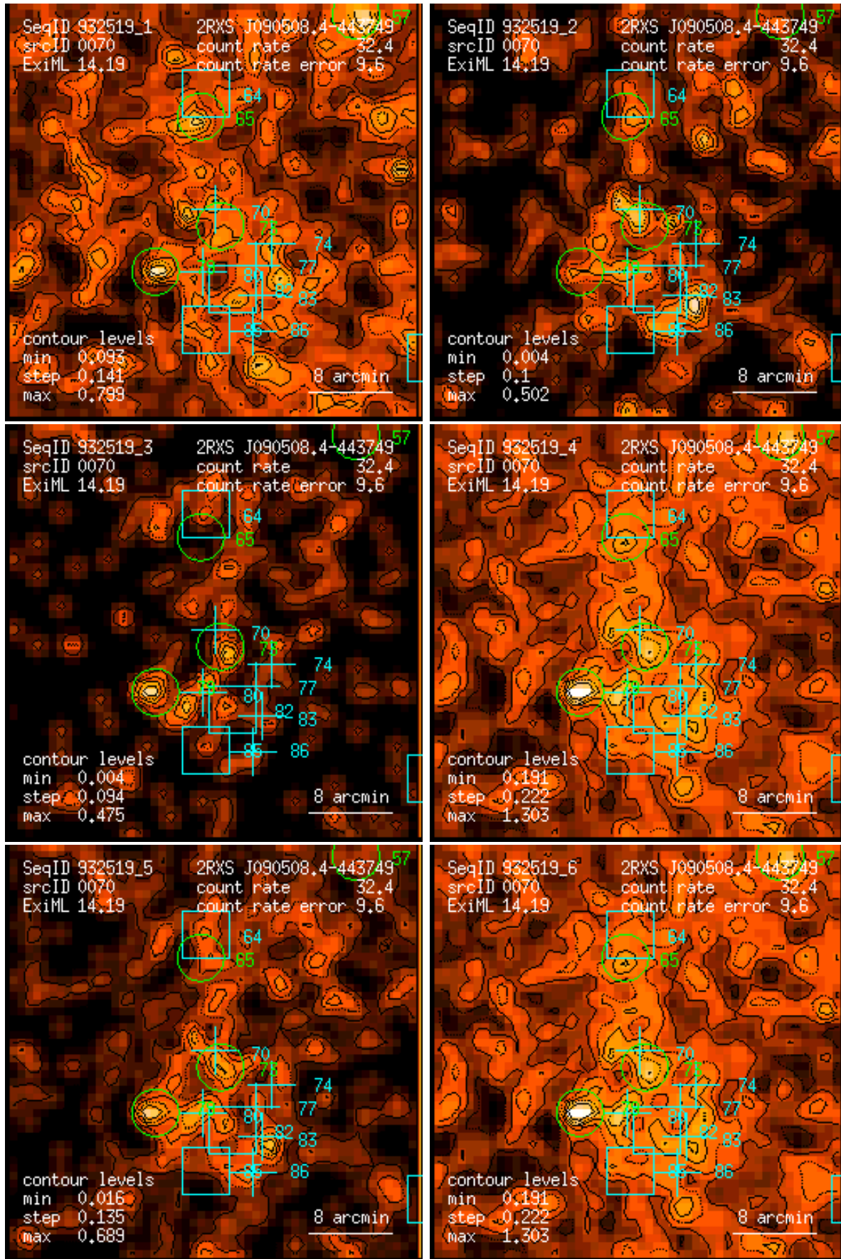
Figure 70: RASS 932519: detection 0070: band rate images, Gaussian filter: (1) PSPC channels 11 – 41, (2) 52 – 90, (3) 91 – 201, (4) 11 – 235, (5) 52 – 201, (6) 11 – 201. Broad band rates in counts/ks. Band rate contour levels in counts/ks/arcmin 2 .
