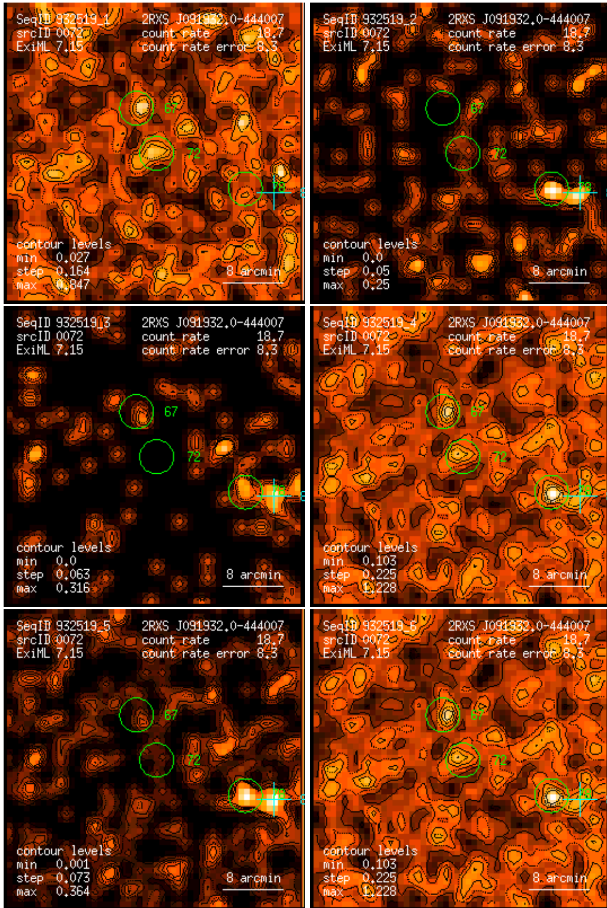
Figure 72: RASS 932519: detection 0072: band rate images, Gaussian filter: (1) PSPC channels 11 – 41, (2) 52 – 90, (3) 91 – 201, (4) 11 – 235, (5) 52 – 201, (6) 11 – 201. Broad band rates in counts/ks. Band rate contour levels in counts/ks/arcmin 2 .
