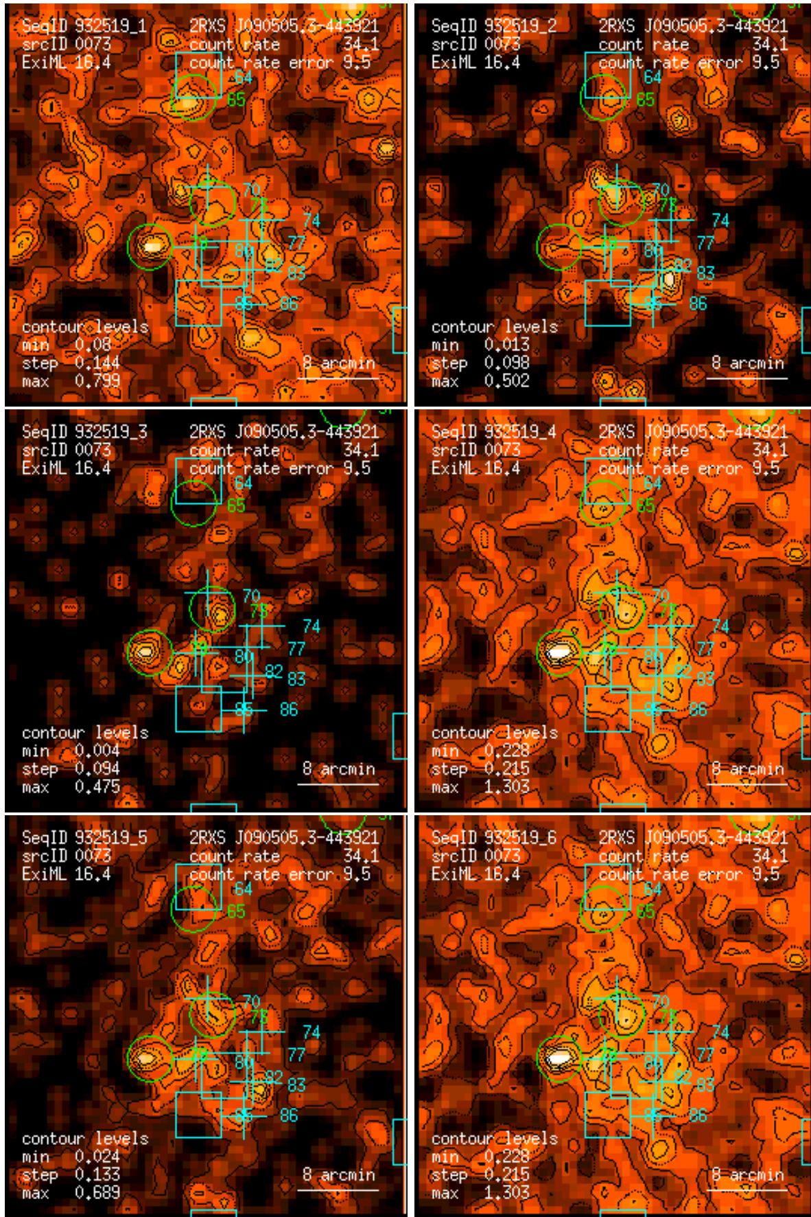
Figure 73: RASS 932519: detection 0073: band rate images, Gaussian filter: (1) PSPC channels 11 – 41, (2) 52 – 90, (3) 91 – 201, (4) 11 – 235, (5) 52 – 201, (6) 11 – 201. Broad band rates in counts/ks. Band rate contour levels in counts/ks/arcmin 2 .
