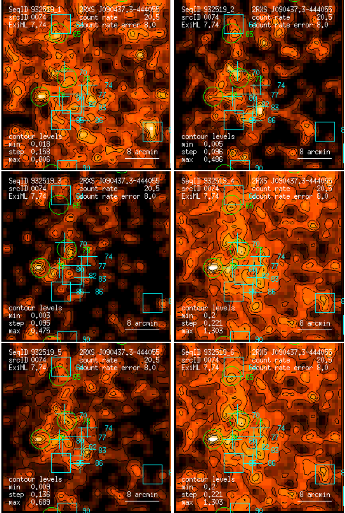
Figure 74: RASS 932519: detection 0074: band rate images, Gaussian filter: (1) PSPC channels 11 – 41, (2) 52 – 90, (3) 91 – 201, (4) 11 – 235, (5) 52 – 201, (6) 11 – 201. Broad band rates in counts/ks. Band rate contour levels in counts/ks/arcmin 2 .
