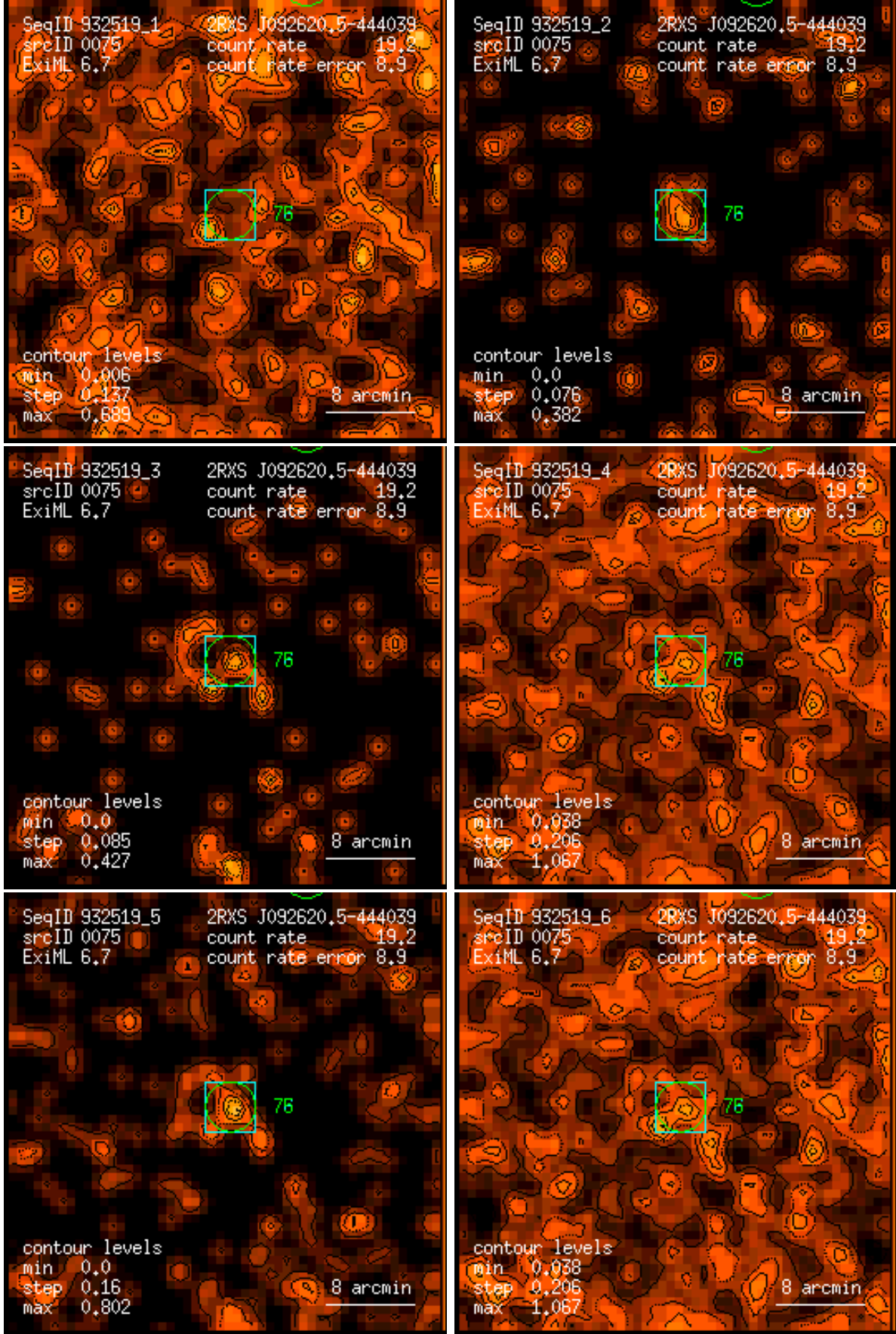
Figure 75: RASS 932519: detection 0075: band rate images, Gaussian filter: (1) PSPC channels 11 – 41, (2) 52 – 90, (3) 91 – 201, (4) 11 – 235, (5) 52 – 201, (6) 11 – 201. Broad band rates in counts/ks. Band rate contour levels in counts/ks/arcmin 2 .
