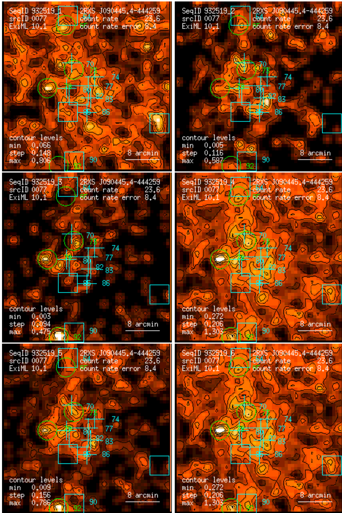
Figure 77: RASS 932519: detection 0077: band rate images, Gaussian filter: (1) PSPC channels 11 – 41, (2) 52 – 90, (3) 91 – 201, (4) 11 – 235, (5) 52 – 201, (6) 11 – 201. Broad band rates in counts/ks. Band rate contour levels in counts/ks/arcmin 2 .
