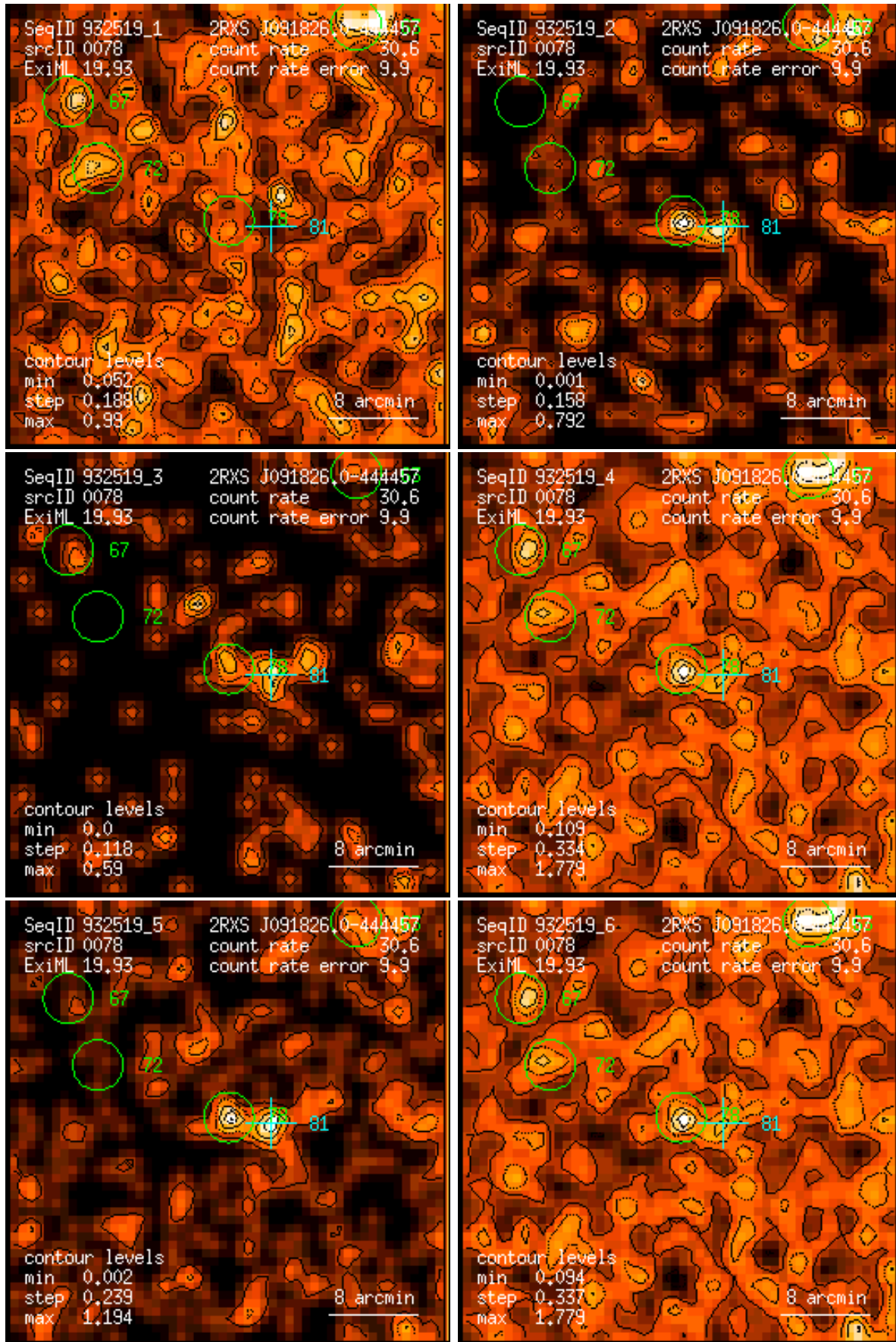
Figure 78: RASS 932519: detection 0078: band rate images, Gaussian filter: (1) PSPC channels 11 – 41, (2) 52 – 90, (3) 91 – 201, (4) 11 – 235, (5) 52 – 201, (6) 11 – 201. Broad band rates in counts/ks. Band rate contour levels in counts/ks/arcmin 2 .
