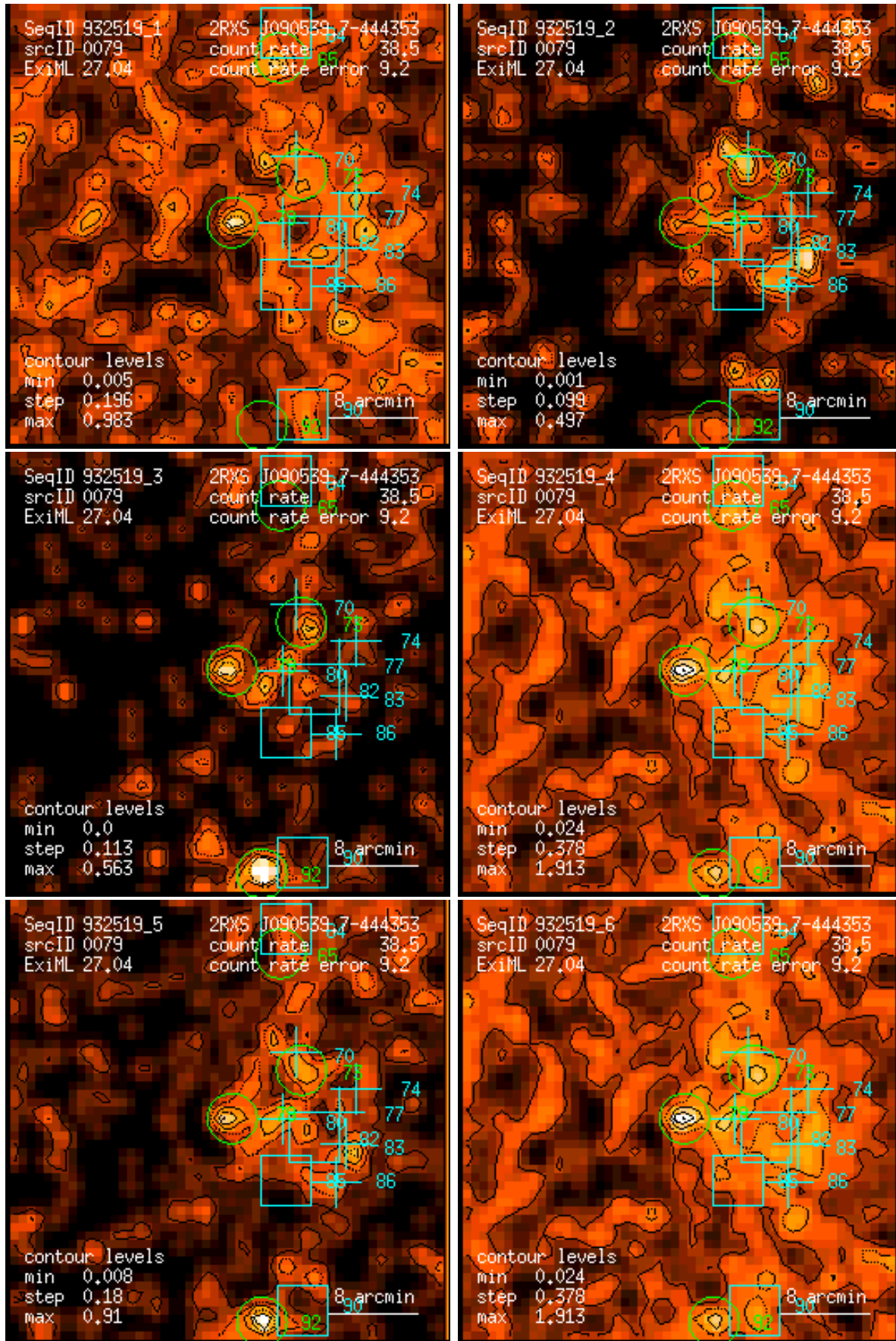
Figure 79: RASS 932519: detection 0079: band rate images, Gaussian filter: (1) PSPC channels 11 – 41, (2) 52 – 90, (3) 91 – 201, (4) 11 – 235, (5) 52 – 201, (6) 11 – 201. Broad band rates in counts/ks. Band rate contour levels in counts/ks/arcmin 2 .
