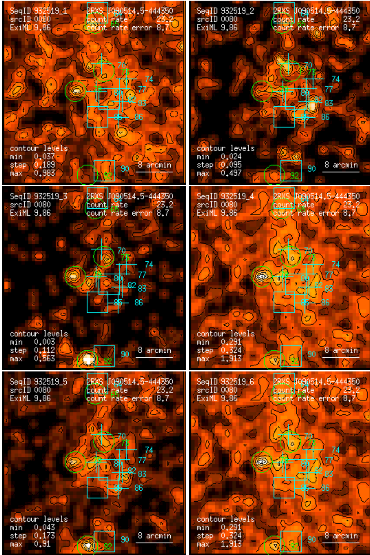
Figure 80: RASS 932519: detection 0080: band rate images, Gaussian filter: (1) PSPC channels 11 – 41, (2) 52 – 90, (3) 91 – 201, (4) 11 – 235, (5) 52 – 201, (6) 11 – 201. Broad band rates in counts/ks. Band rate contour levels in counts/ks/arcmin 2 .
