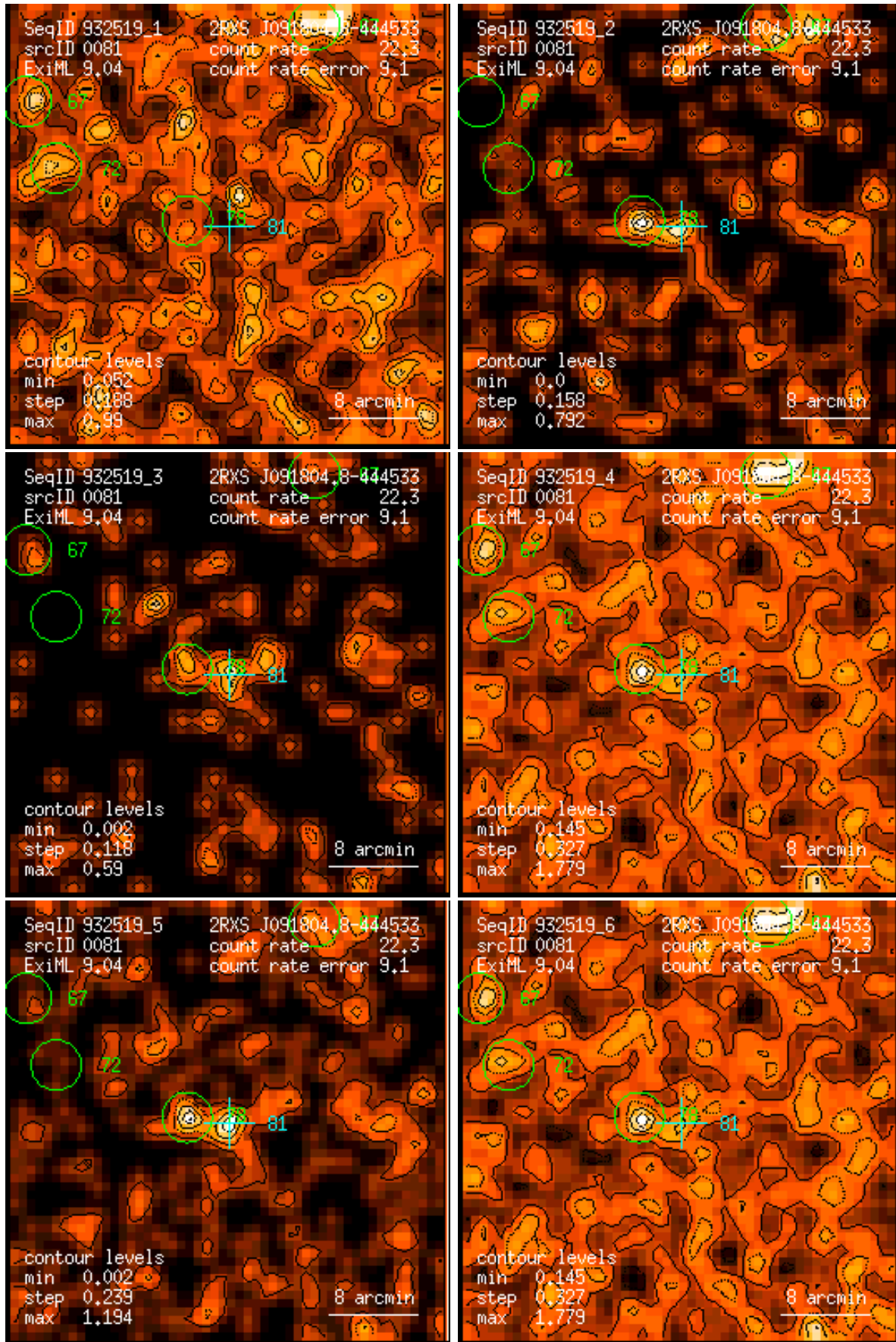
Figure 81: RASS 932519: detection 0081: band rate images, Gaussian filter: (1) PSPC channels 11 – 41, (2) 52 – 90, (3) 91 – 201, (4) 11 – 235, (5) 52 – 201, (6) 11 – 201. Broad band rates in counts/ks. Band rate contour levels in counts/ks/arcmin 2 .
