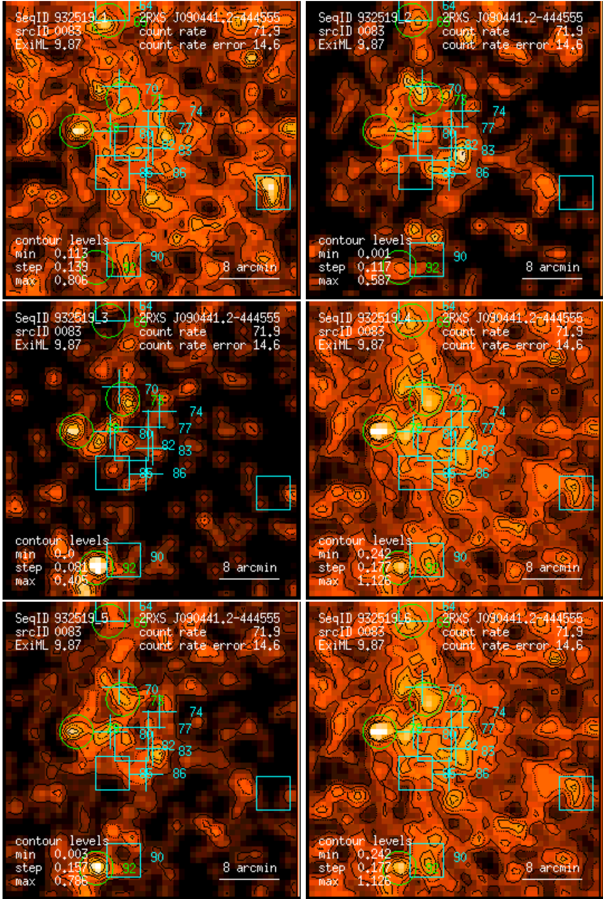
Figure 83: RASS 932519: detection 0083: band rate images, Gaussian filter: (1) PSPC channels 11 – 41, (2) 52 – 90, (3) 91 – 201, (4) 11 – 235, (5) 52 – 201, (6) 11 – 201. Broad band rates in counts/ks. Band rate contour levels in counts/ks/arcmin 2 .
