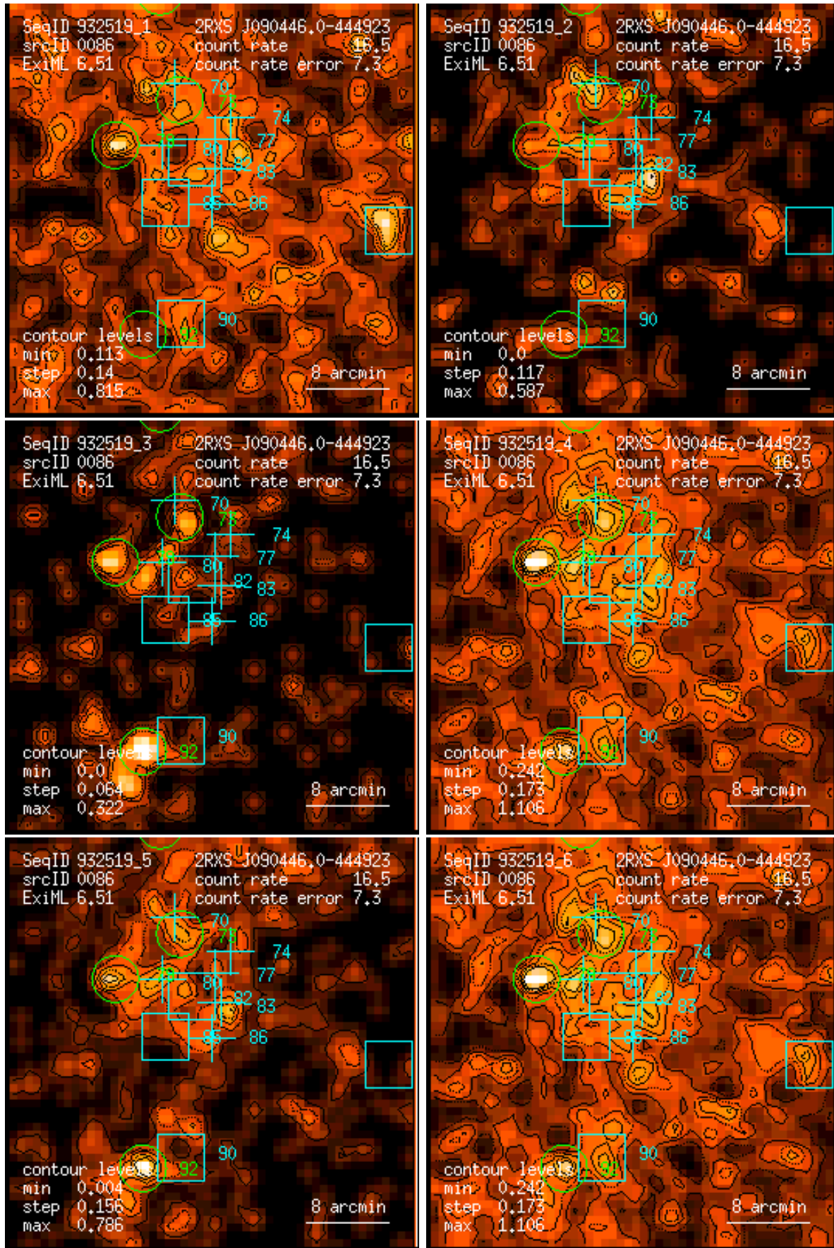
Figure 86: RASS 932519: detection 0086: band rate images, Gaussian filter: (1) PSPC channels 11 – 41, (2) 52 – 90, (3) 91 – 201, (4) 11 – 235, (5) 52 – 201, (6) 11 – 201. Broad band rates in counts/ks. Band rate contour levels in counts/ks/arcmin 2 .
