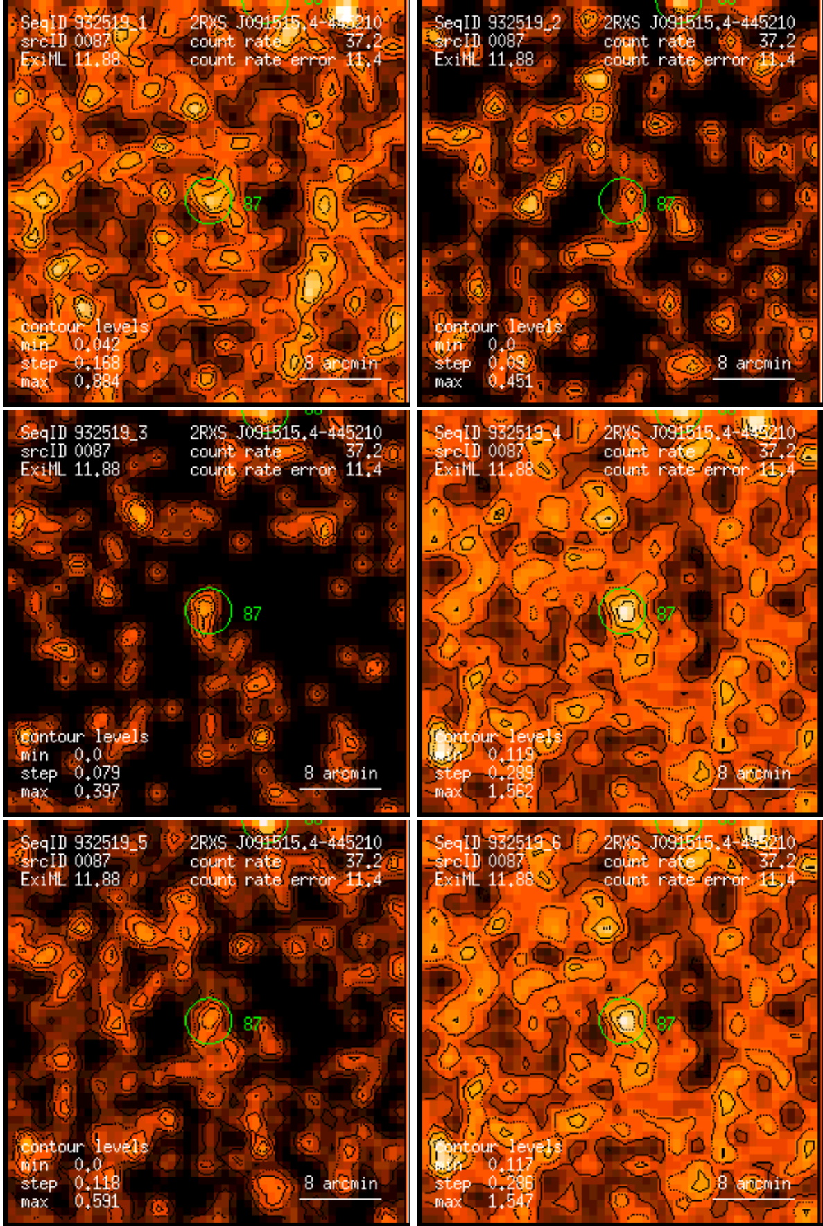
Figure 87: RASS 932519: detection 0087: band rate images, Gaussian filter: (1) PSPC channels 11 – 41, (2) 52 – 90, (3) 91 – 201, (4) 11 – 235, (5) 52 – 201, (6) 11 – 201. Broad band rates in counts/ks. Band rate contour levels in counts/ks/arcmin 2 .
