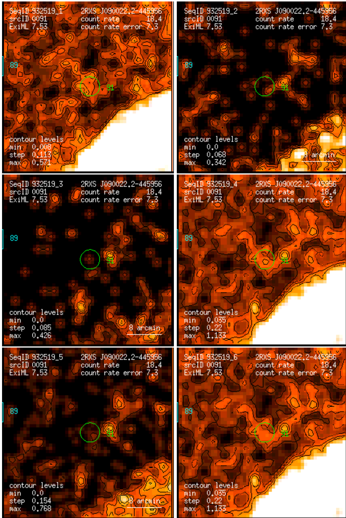
Figure 91: RASS 932519: detection 0091: band rate images, Gaussian filter: (1) PSPC channels 11 – 41, (2) 52 – 90, (3) 91 – 201, (4) 11 – 235, (5) 52 – 201, (6) 11 – 201. Broad band rates in counts/ks. Band rate contour levels in counts/ks/arcmin 2 .
