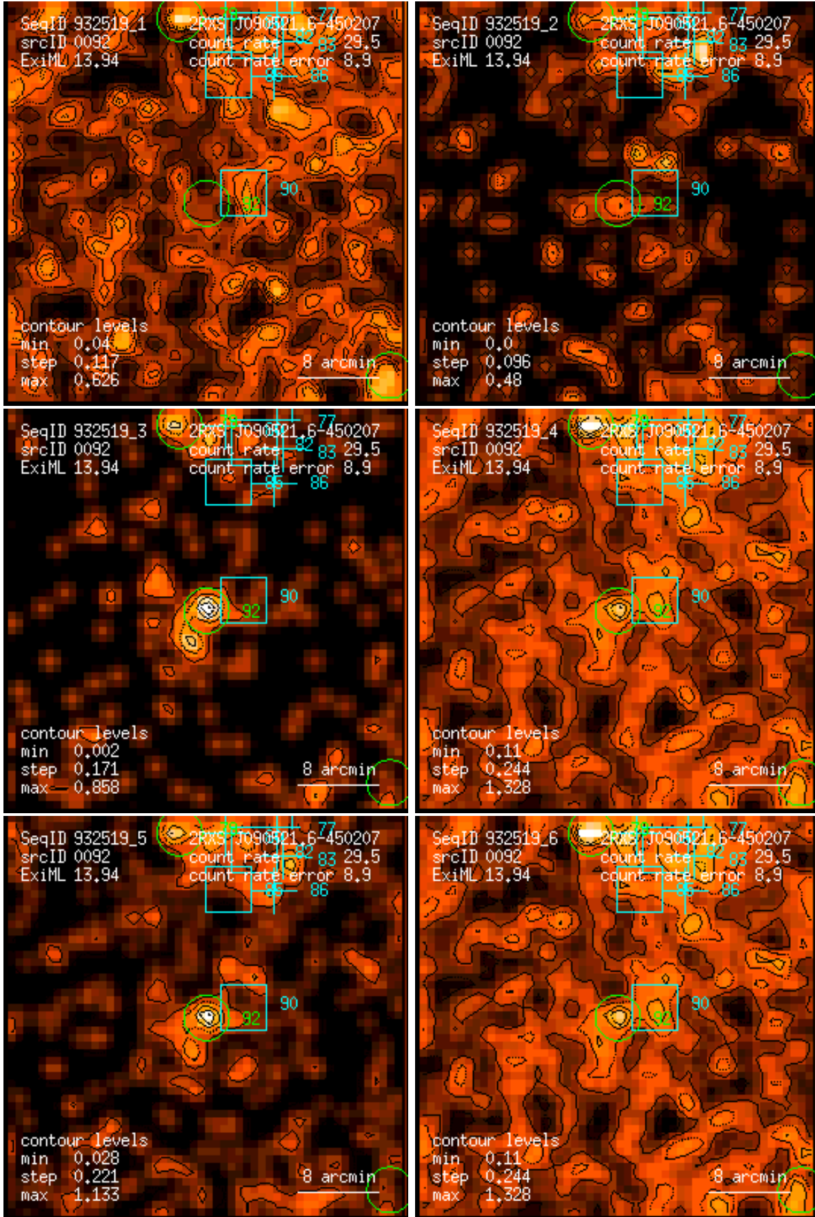
Figure 92: RASS 932519: detection 0092: band rate images, Gaussian filter: (1) PSPC channels 11 – 41, (2) 52 – 90, (3) 91 – 201, (4) 11 – 235, (5) 52 – 201, (6) 11 – 201. Broad band rates in counts/ks. Band rate contour levels in counts/ks/arcmin 2 .
