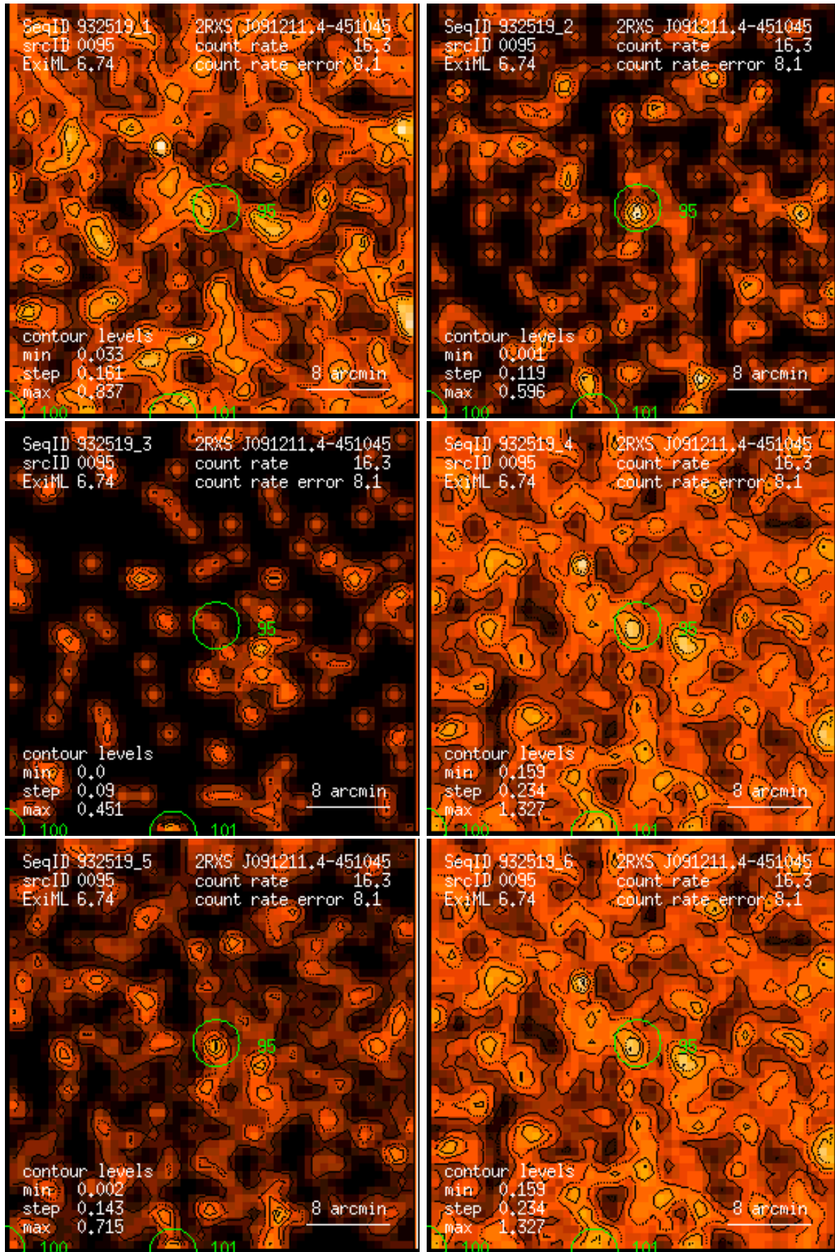
Figure 95: RASS 932519: detection 0095: band rate images, Gaussian filter: (1) PSPC channels 11 – 41, (2) 52 – 90, (3) 91 – 201, (4) 11 – 235, (5) 52 – 201, (6) 11 – 201. Broad band rates in counts/ks. Band rate contour levels in counts/ks/arcmin 2 .
