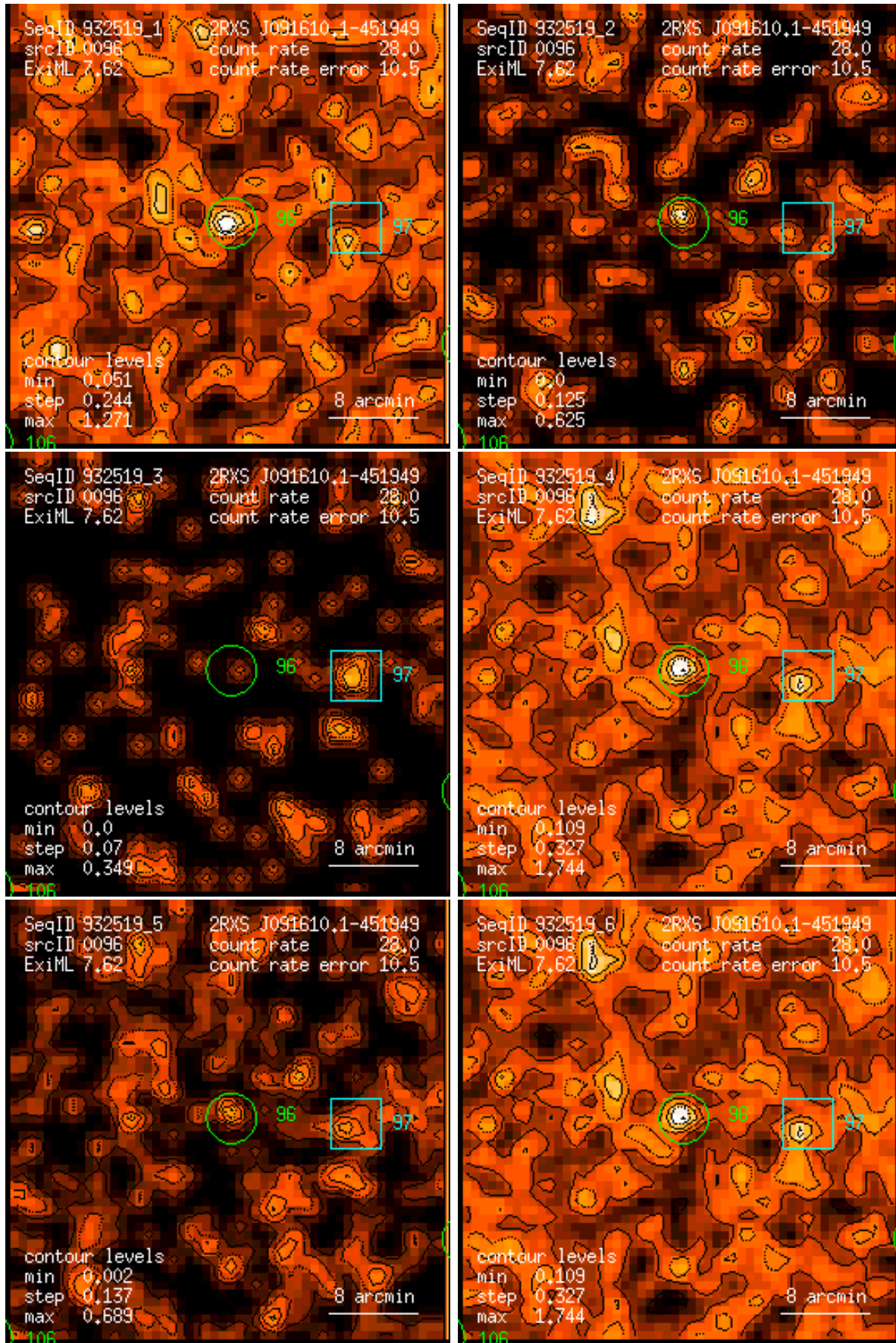
Figure 96: RASS 932519: detection 0096: band rate images, Gaussian filter: (1) PSPC channels 11 – 41, (2) 52 – 90, (3) 91 – 201, (4) 11 – 235, (5) 52 – 201, (6) 11 – 201. Broad band rates in counts/ks. Band rate contour levels in counts/ks/arcmin 2 .
