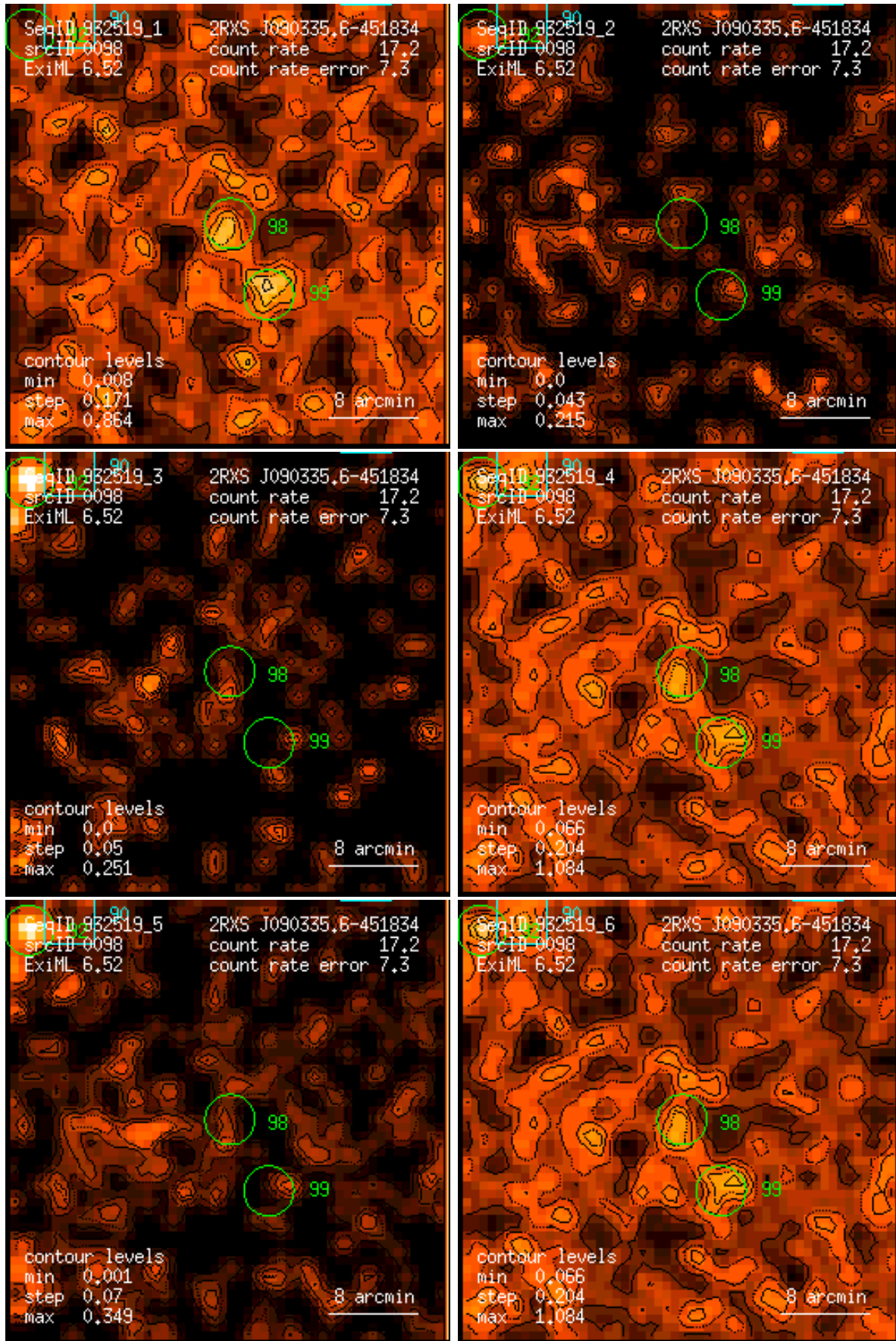
Figure 98: RASS 932519: detection 0098: band rate images, Gaussian filter: (1) PSPC channels 11 – 41, (2) 52 – 90, (3) 91 – 201, (4) 11 – 235, (5) 52 – 201, (6) 11 – 201. Broad band rates in counts/ks. Band rate contour levels in counts/ks/arcmin 2 .
