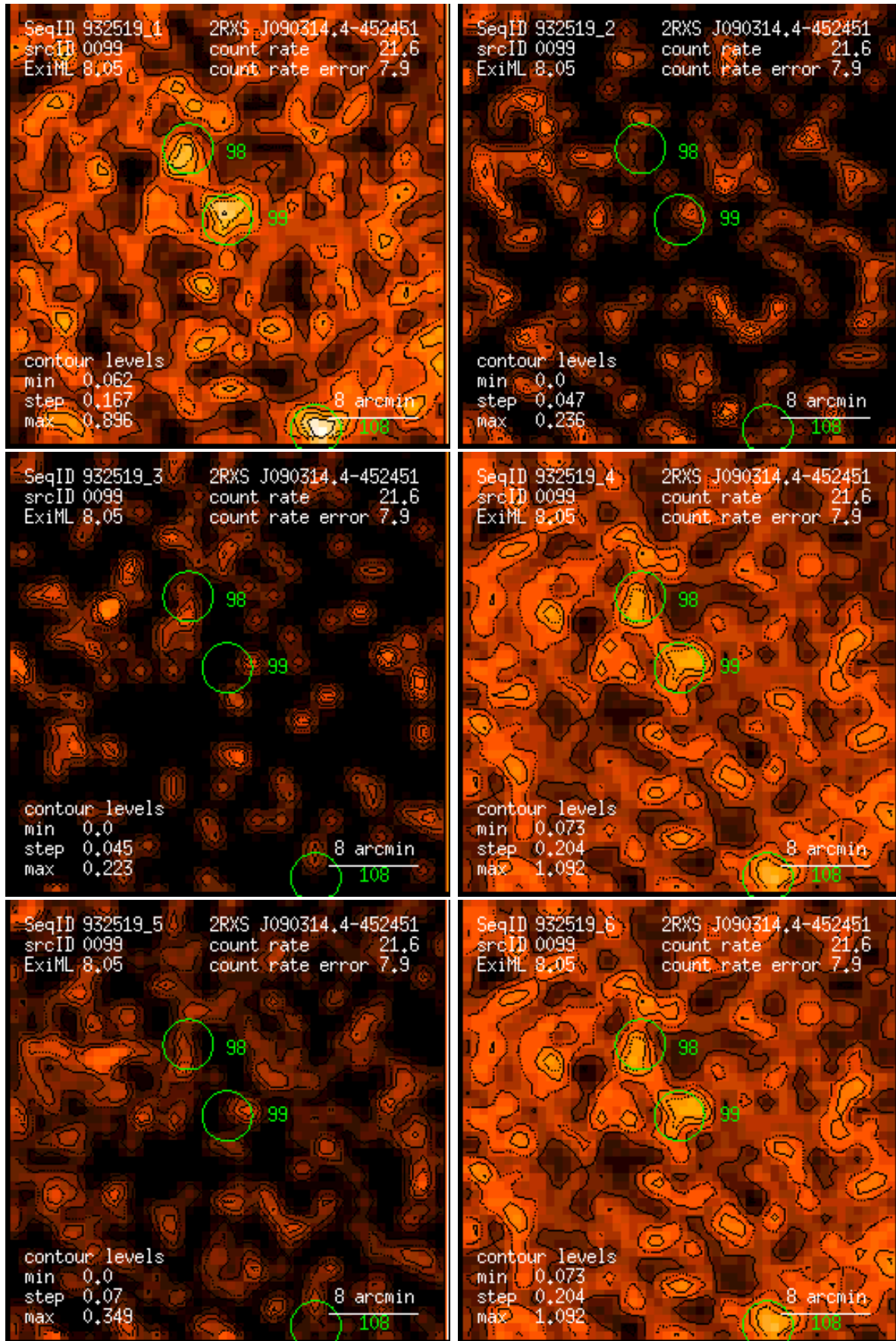
Figure 99: RASS 932519: detection 0099: band rate images, Gaussian filter: (1) PSPC channels 11 – 41, (2) 52 – 90, (3) 91 – 201, (4) 11 – 235, (5) 52 – 201, (6) 11 – 201. Broad band rates in counts/ks. Band rate contour levels in counts/ks/arcmin 2 .
