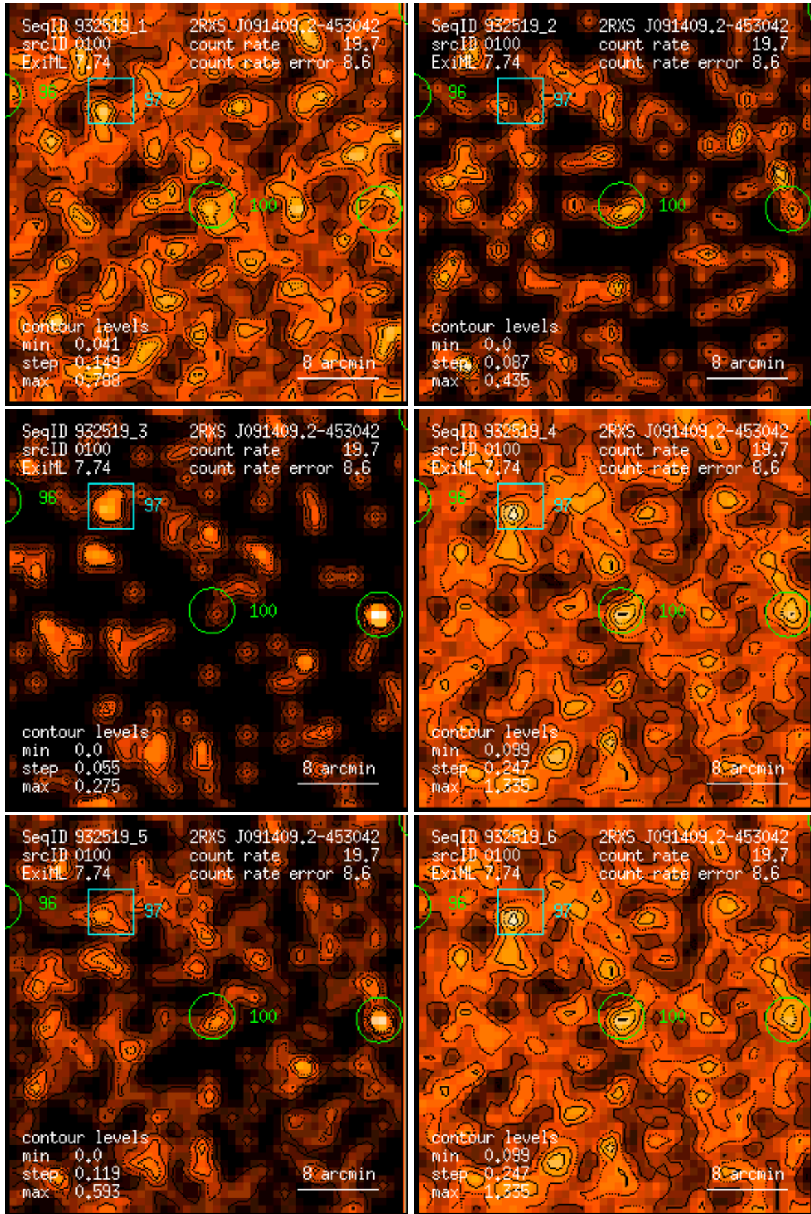
Figure 100: RASS 932519: detection 0100: band rate images, Gaussian filter: (1) PSPC channels 11 – 41, (2) 52 – 90, (3) 91 – 201, (4) 11 – 235, (5) 52 – 201, (6) 11 – 201. Broad band rates in counts/ks. Band rate contour levels in counts/ks/arcmin 2 .
