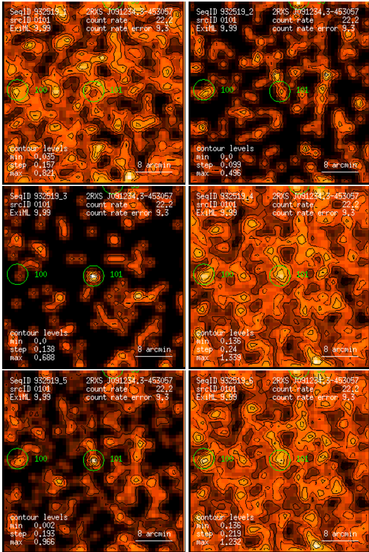
Figure 101: RASS 932519: detection 0101: band rate images, Gaussian filter: (1) PSPC channels 11 – 41, (2) 52 – 90, (3) 91 – 201, (4) 11 – 235, (5) 52 – 201, (6) 11 – 201. Broad band rates in counts/ks. Band rate contour levels in counts/ks/arcmin 2 .
