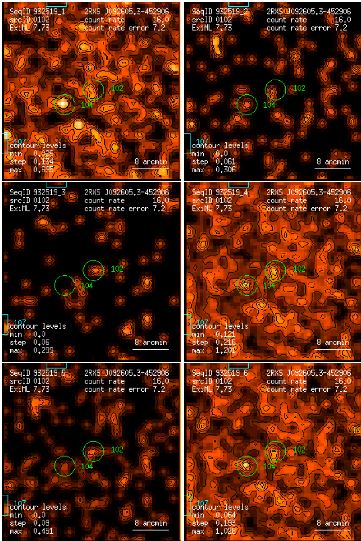
Figure 102: RASS 932519: detection 0102: band rate images, Gaussian filter: (1) PSPC channels 11 – 41, (2) 52 – 90, (3) 91 – 201, (4) 11 – 235, (5) 52 – 201, (6) 11 – 201. Broad band rates in counts/ks. Band rate contour levels in counts/ks/arcmin 2 .
