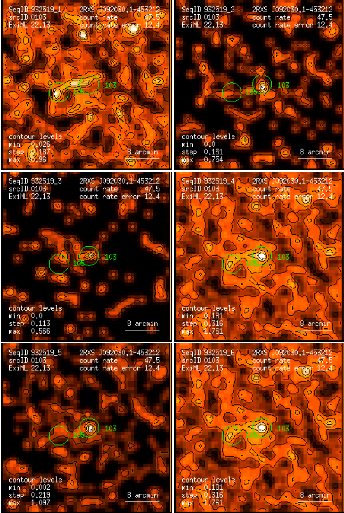
Figure 103: RASS 932519: detection 0103: band rate images, Gaussian filter: (1) PSPC channels 11 – 41, (2) 52 – 90, (3) 91 – 201, (4) 11 – 235, (5) 52 – 201, (6) 11 – 201. Broad band rates in counts/ks. Band rate contour levels in counts/ks/arcmin 2 .
