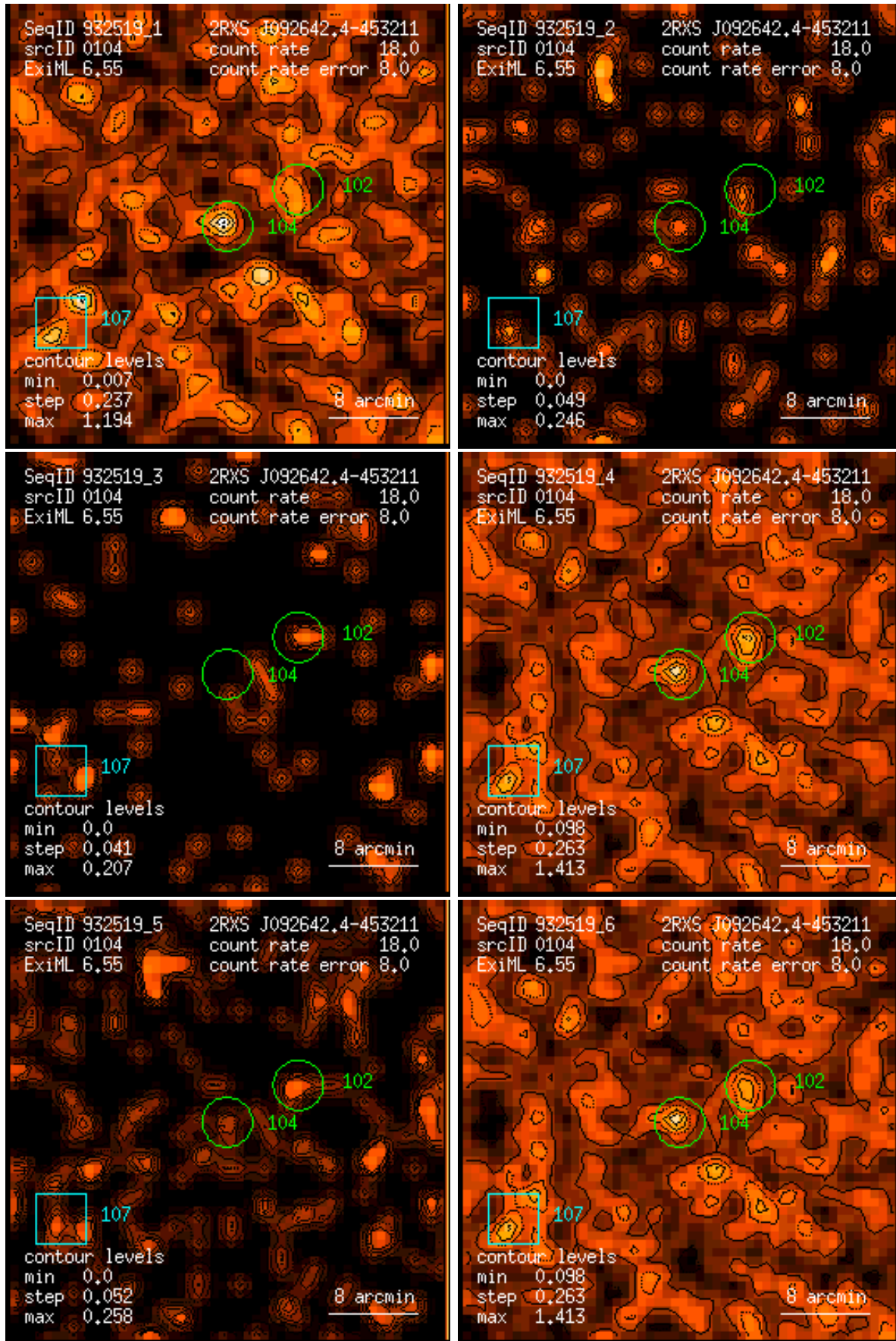
Figure 104: RASS 932519: detection 0104: band rate images, Gaussian filter: (1) PSPC channels 11 – 41, (2) 52 – 90, (3) 91 – 201, (4) 11 – 235, (5) 52 – 201, (6) 11 – 201. Broad band rates in counts/ks. Band rate contour levels in counts/ks/arcmin 2 .
